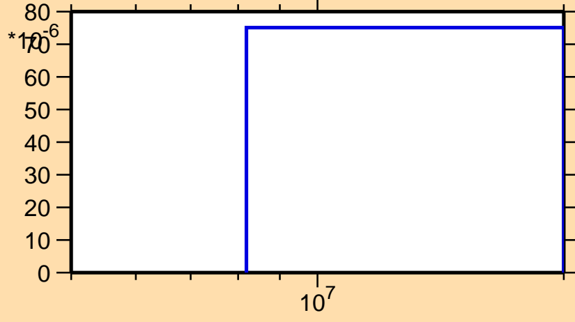
\sigma vs. E for ^{190}\text{Os}(n,d)
