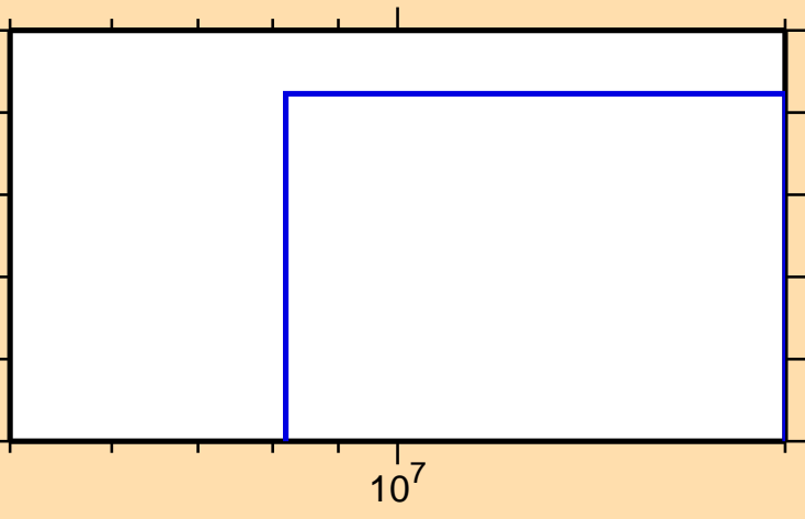
\sigma vs. E for ^{190}\text{Os}(n,3n)
