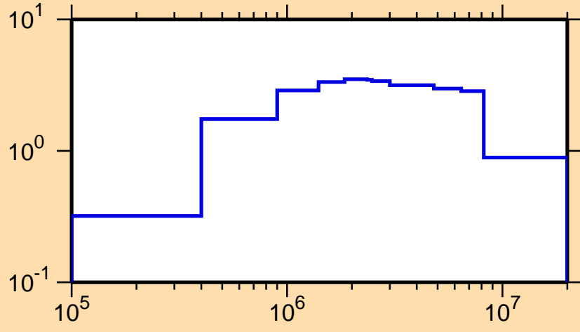
\sigma vs. E for ^{190}\text{Os}(n,\text{inel.})
