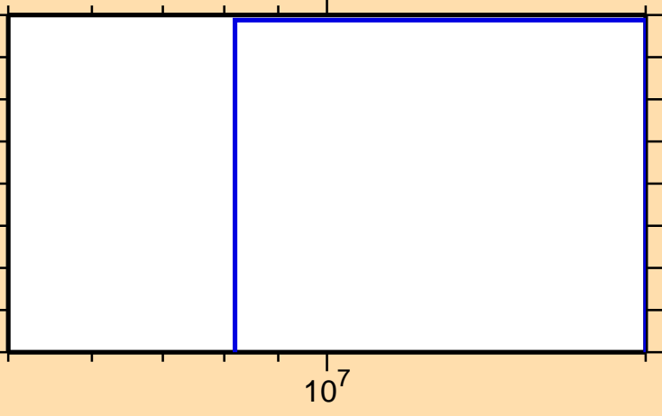
\sigma vs. E for ^{191}\text{Os}(n,3n)
