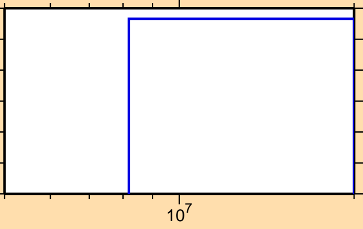
\sigma vs. E for ^{191}\text{Os}(n,t)
