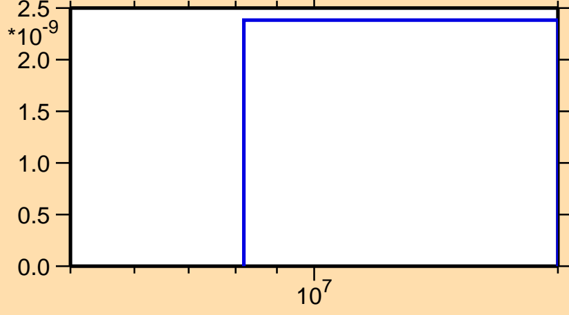
\sigma vs. E for ^{191}\text{Os}(n,2n\alpha)
