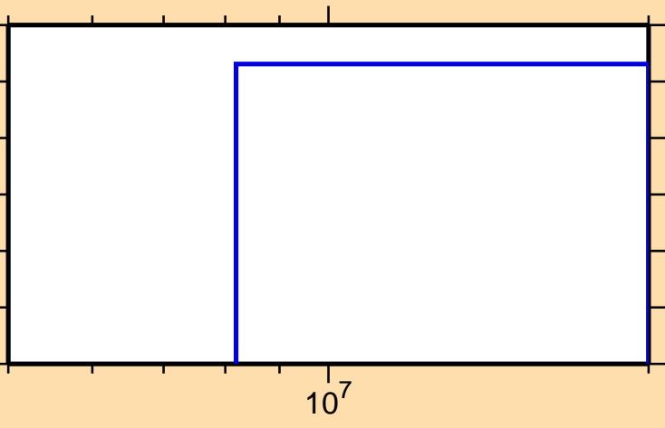
\sigma vs. E for ^{192}\text{Os}(n,\text{He}3)
