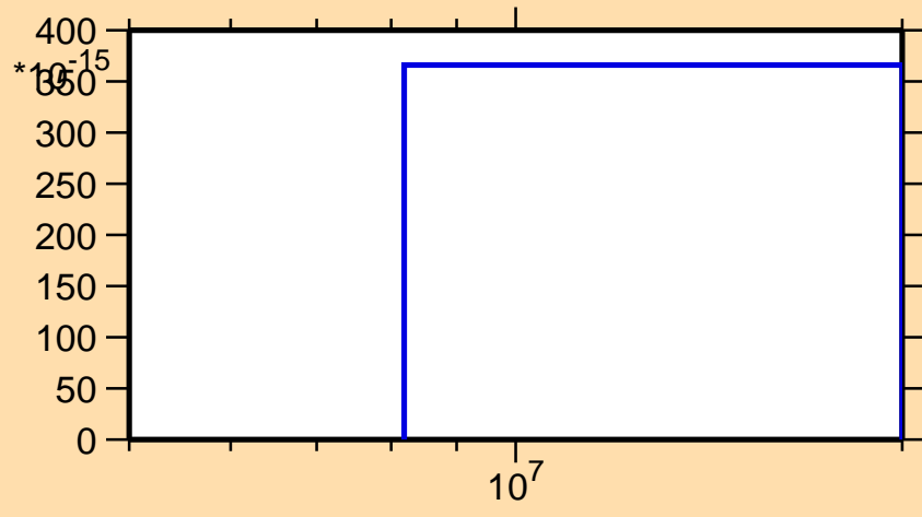
\sigma vs. E for ^{192}\text{Os}(n,2np)
