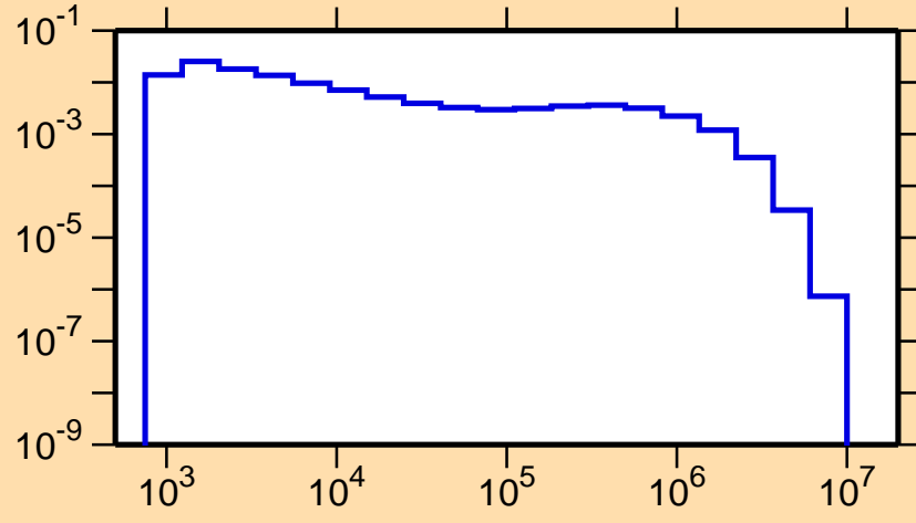
\sigma vs. E for ^{192}\text{Os}(n,n_4)
