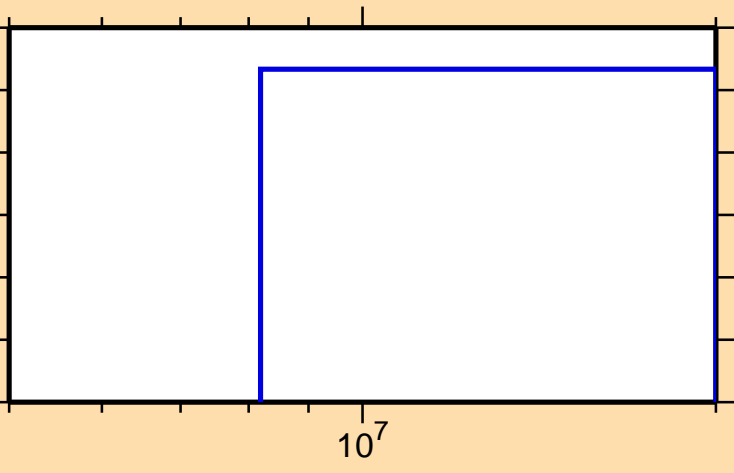
\sigma vs. E for ^{192}\text{Os}(n,\text{nd})
