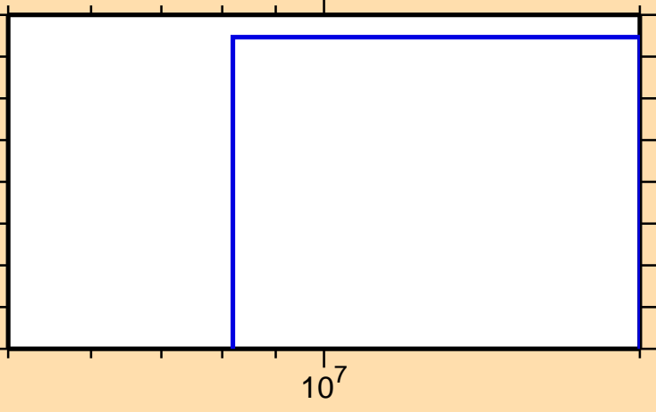
\sigma vs. E for ^{192}\text{Os}(n,t)
