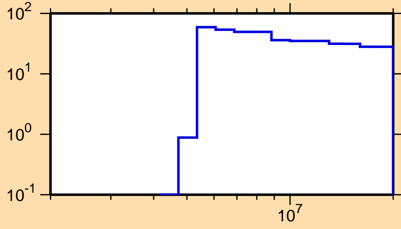
\Delta\sigma/\sigma vs. E for ^{193}\text{Os}(n,p)
