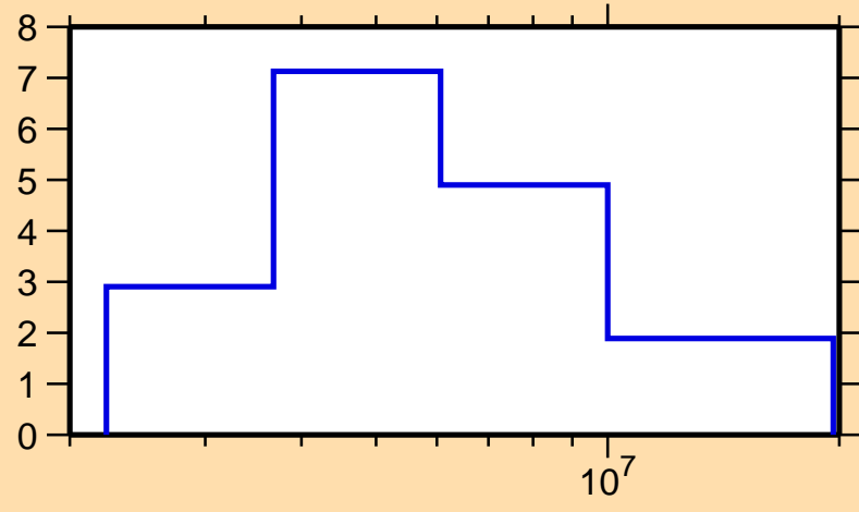
\Delta\sigma/\sigma vs. E for ^{193}\text{Os}(n,\text{el.})
