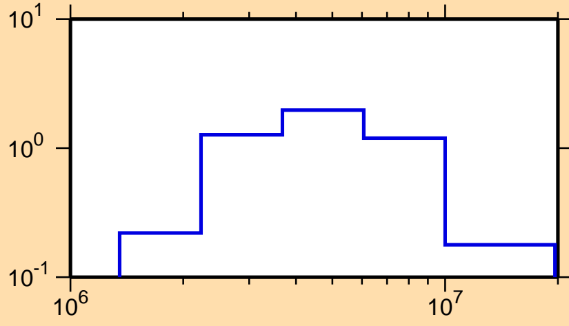
\sigma vs. E for ^{193}\text{Os}(n,n\text{cont.})
