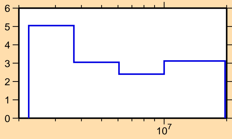
\Delta\sigma/\sigma vs. E for ^{193}\text{Os}(n,\text{nonel.})
