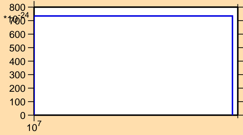
\sigma vs. E for ^{193}\text{Os} (mt 11)
