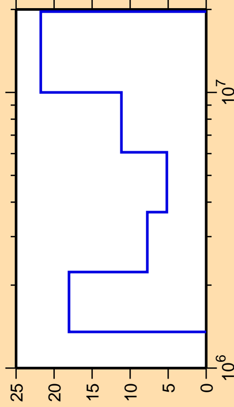
\Delta\sigma/\sigma vs. E for ^{193}\text{Os}(n,n\text{cont.})
