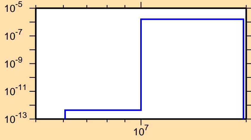
\sigma vs. E for ^{193}\text{Os}(n,n\alpha)
