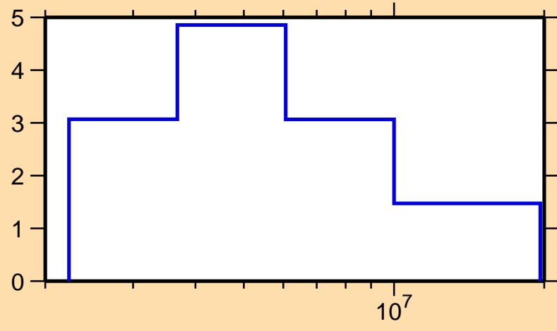
\Delta\sigma/\sigma vs. E for ^{193}\text{Os}(n,\text{tot.})
