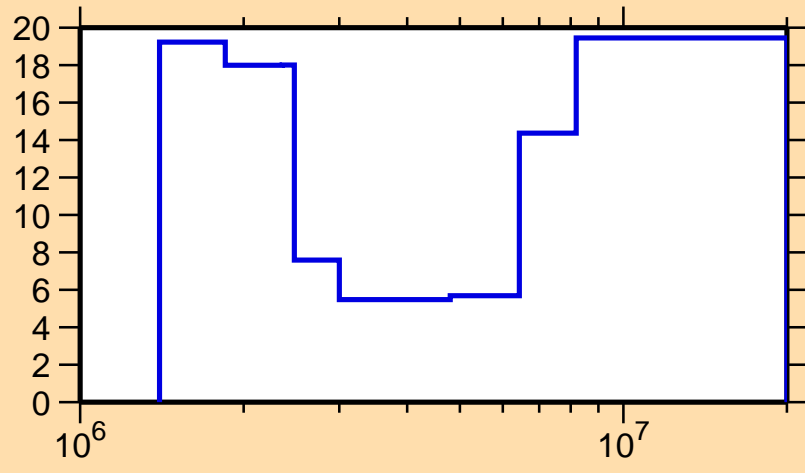
\Delta\sigma/\sigma vs. E for ^{193}\text{Os}(n,n\text{cont.})
