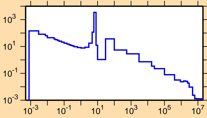
\sigma vs. E for ^{193}\text{Os}(n,\gamma)
