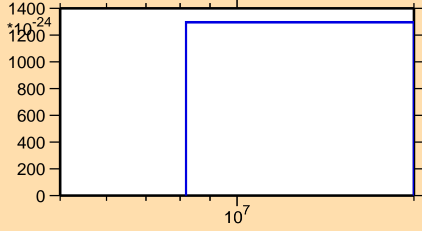
\sigma vs. E for ^{193}\text{Os}(\text{mt } 11)
