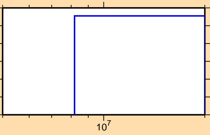
\sigma vs. E for ^{193}\text{Os}(n,np)
