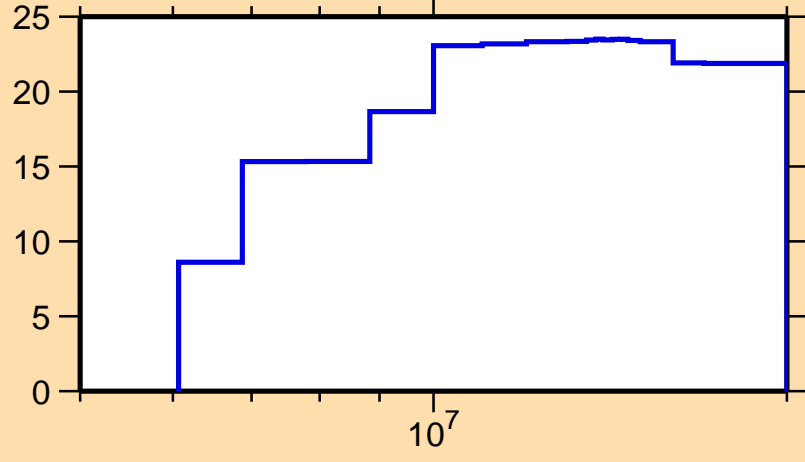
\Delta\sigma/\sigma vs. E for ^{194}\text{Os}(n,ncont.)
