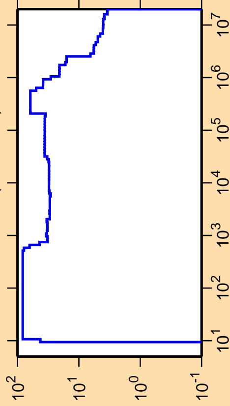
\Delta\sigma/\sigma vs. E for ^{194}\text{Os}(n,\text{nonel.})
