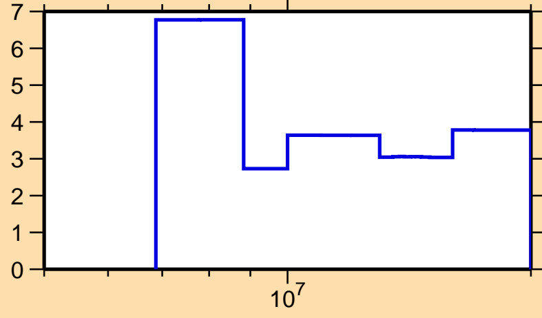
\Delta\sigma/\sigma vs. E for ^{194}\text{Os}(n,\text{el.})
