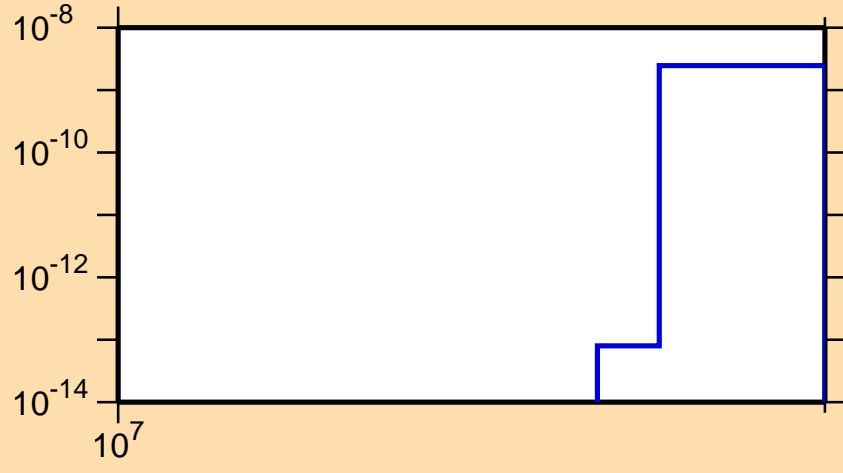
\sigma vs. E for ^{194}\text{Os}(n,nt)
