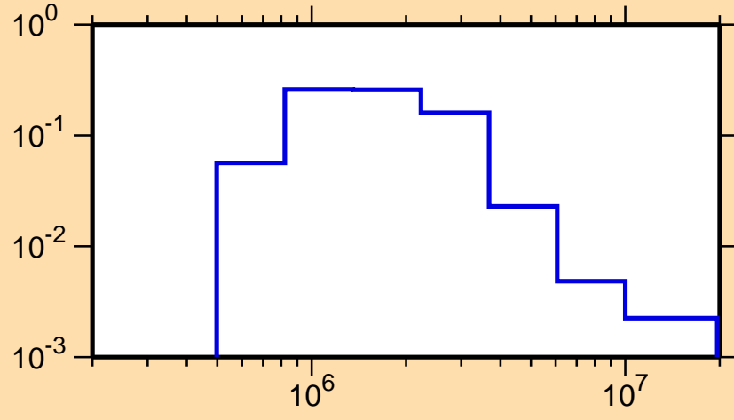
\sigma vs. E for ^{194}\text{Os}(n,n_3)
