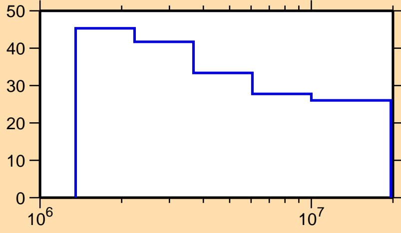
\Delta\sigma/\sigma vs. E for ^{194}\text{Os}(n,n_1)
