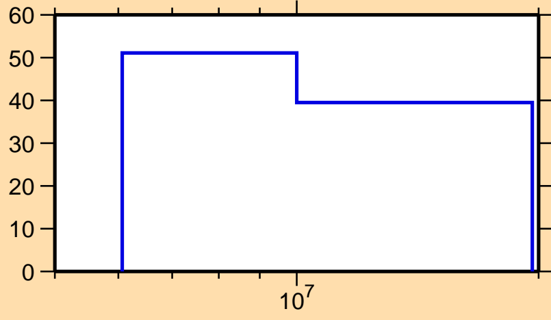
\Delta\sigma/\sigma vs. E for ^{194}\text{Os}(n,p)
