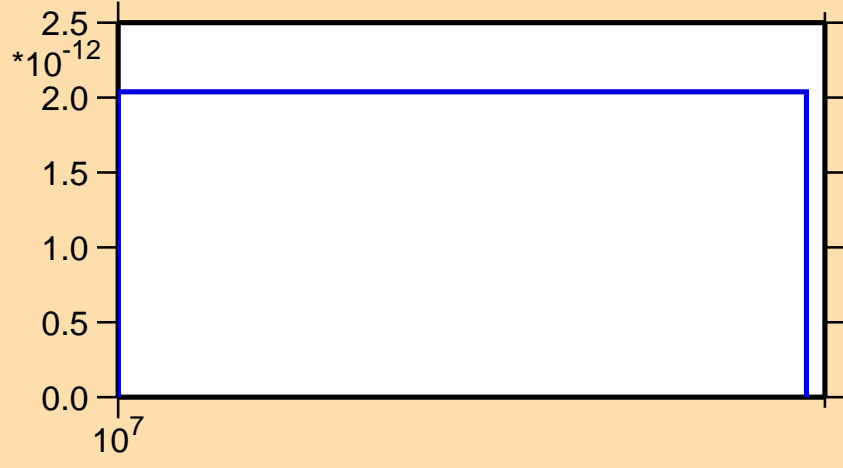
\sigma vs. E for ^{194}\text{Os}(n,\text{nd})
