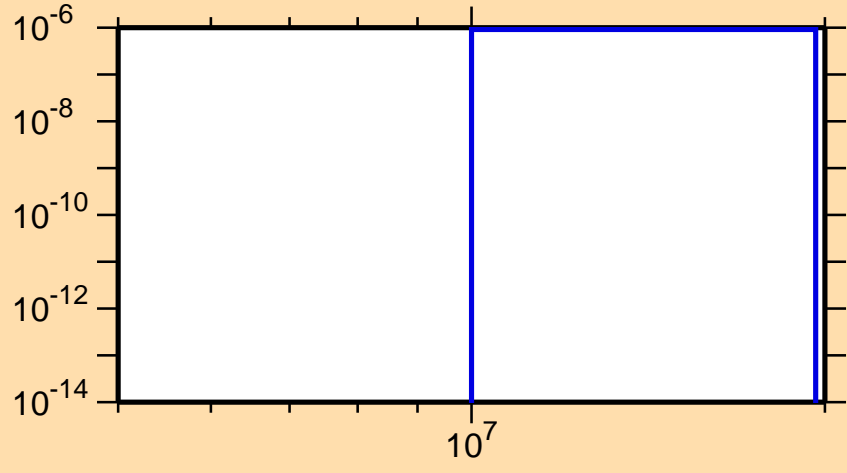
\sigma vs. E for ^{194}\text{Os}(n,t)
