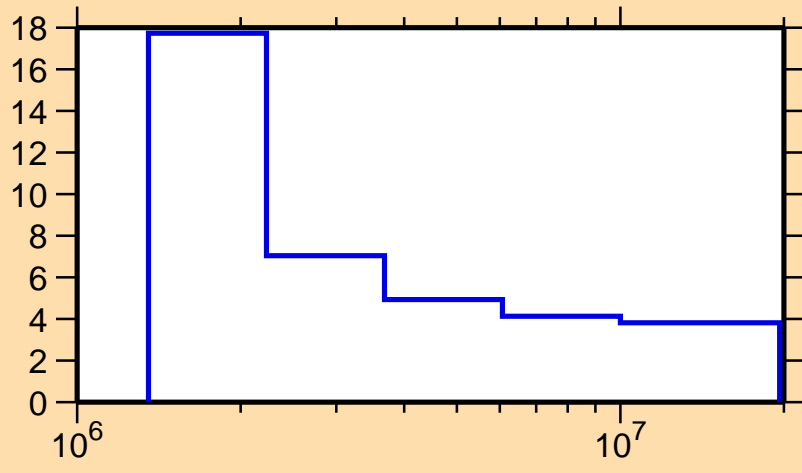
\Delta\sigma/\sigma vs. E for ^{194}\text{Os}(n,\text{nonel.})
