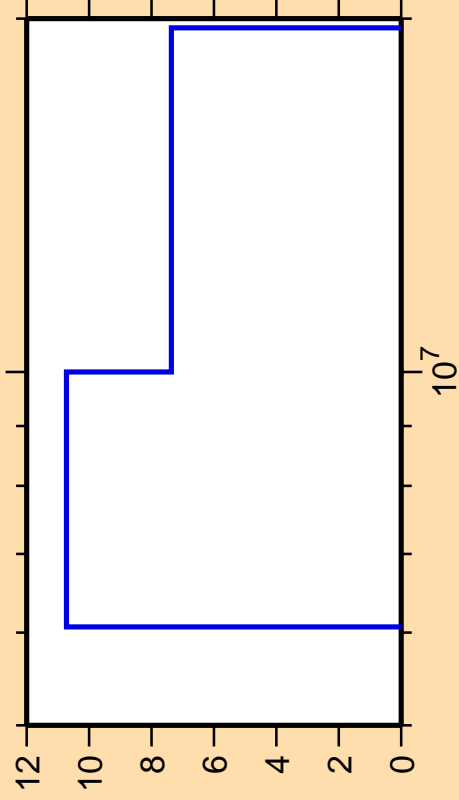
\Delta\sigma/\sigma vs. E for ^{194}\text{Os}(n,2n)
