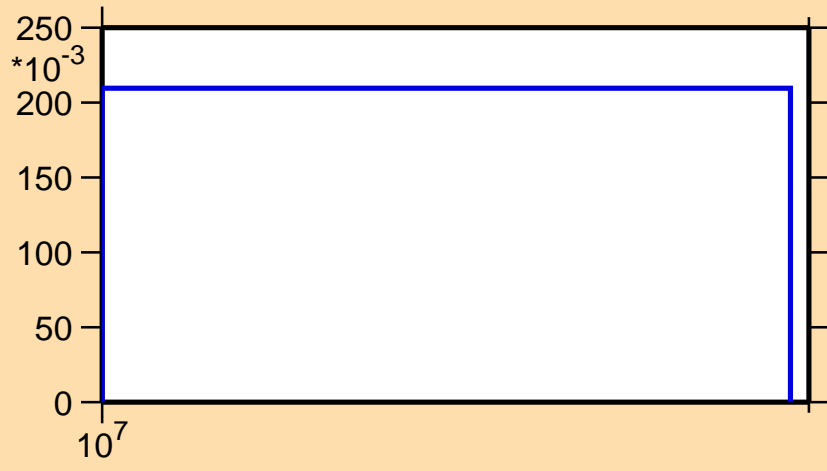
\sigma vs. E for ^{194}\text{Os}(n,3n)
