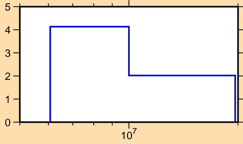
\Delta\sigma/\sigma vs. E for ^{194}\text{Os}(n,\text{tot.})
