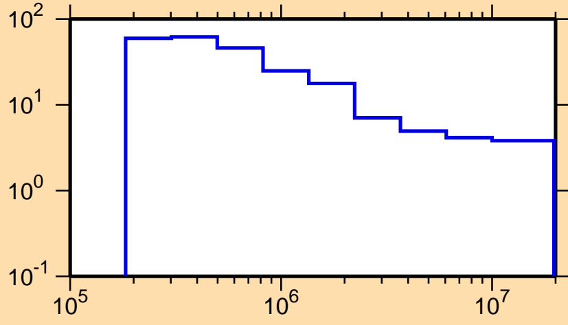
\Delta\sigma/\sigma vs. E for ^{194}\text{Os}(n,\text{nonel.})
