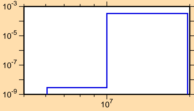
\sigma vs. E for ^{194}\text{Os}(n,p)
