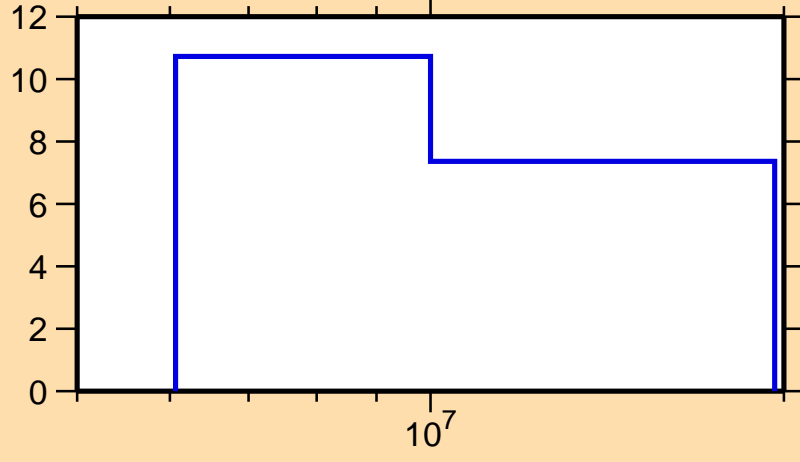
\Delta\sigma/\sigma vs. E for ^{194}\text{Os}(n,2n)
