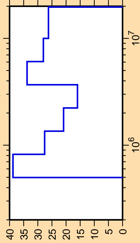
\Delta\sigma/\sigma vs. E for ^{194}\text{Os}(n,n_3)
