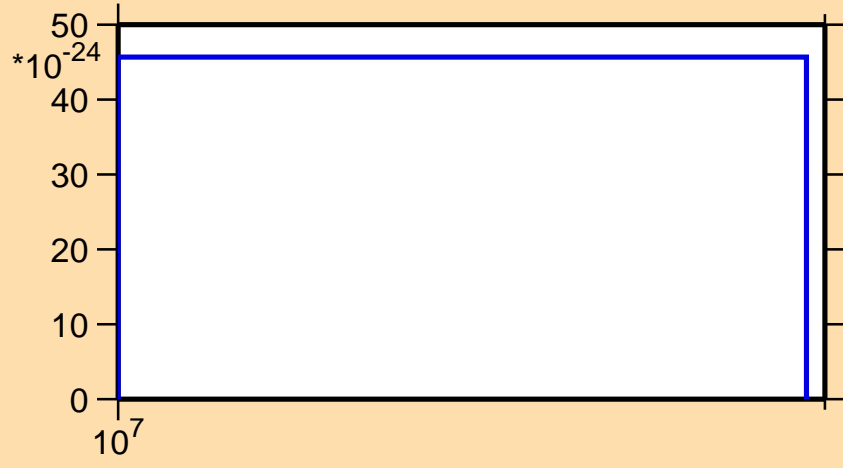
\sigma vs. E for ^{194}\text{Os} (mt 11)
