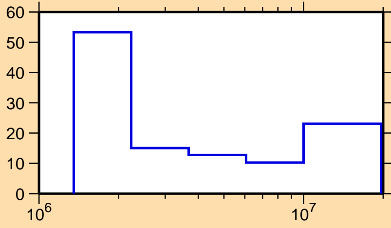
\Delta\sigma/\sigma vs. E for ^{194}\text{Os}(n,n\text{cont.})
