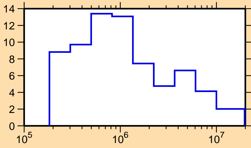
\Delta\sigma/\sigma vs. E for ^{194}\text{Os}(n,\text{tot.})
