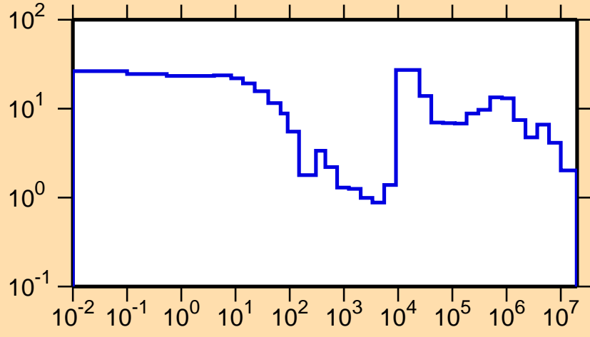
\Delta\sigma/\sigma vs. E for ^{194}\text{Os}(n,\text{tot.})
