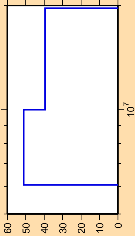
\Delta\sigma/\sigma vs. E for ^{194}\text{Os}(n,p)
