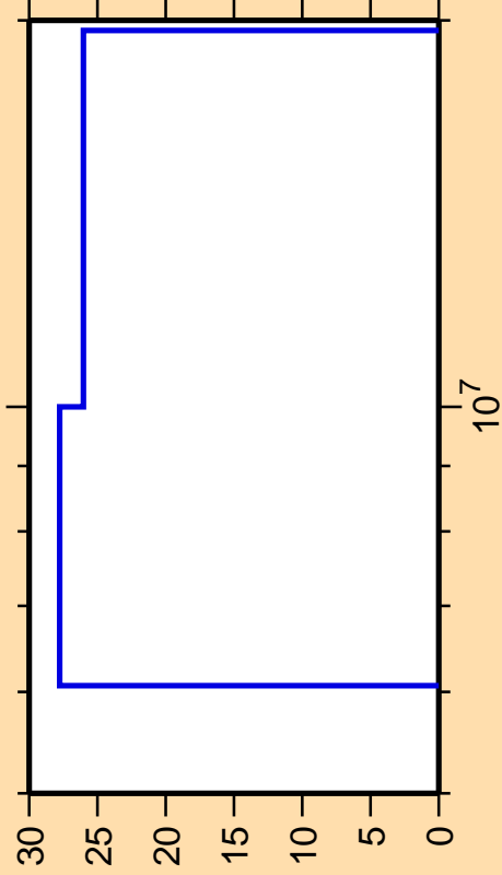
\Delta\sigma/\sigma vs. E for ^{194}\text{Os}(n,n_1)
