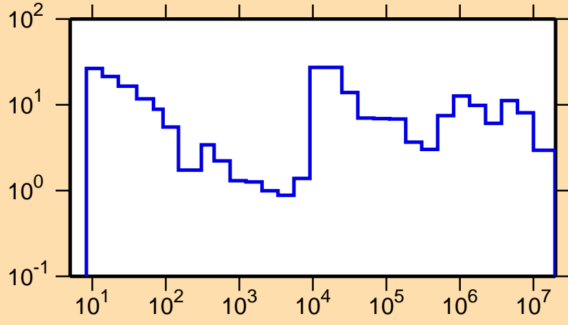
\Delta\sigma/\sigma vs. E for ^{194}\text{Os}(n,\text{el.})
