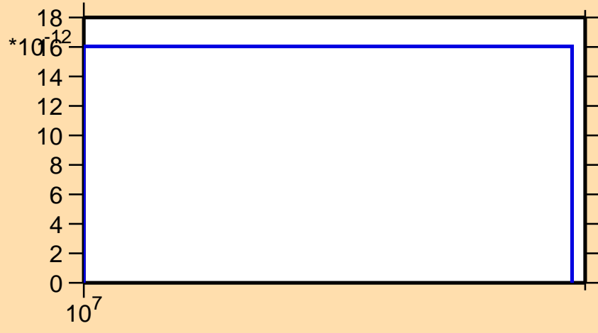
\sigma vs. E for ^{194}\text{Os}(n,nt)
