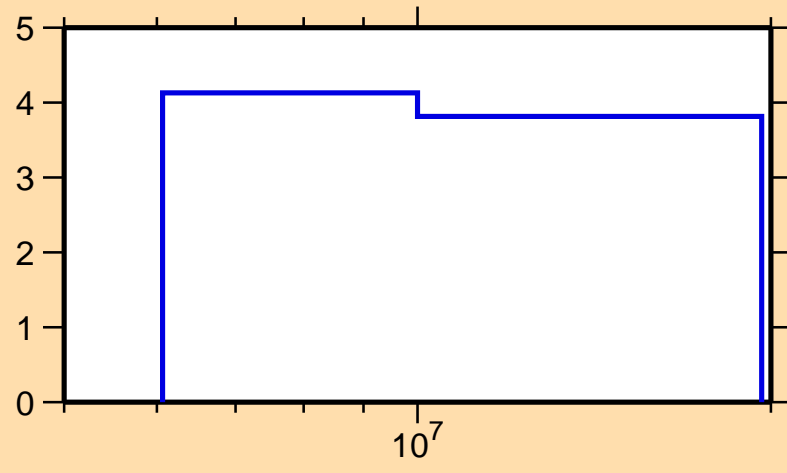
\Delta\sigma/\sigma vs. E for ^{194}\text{Os}(n,\text{nonel.})
