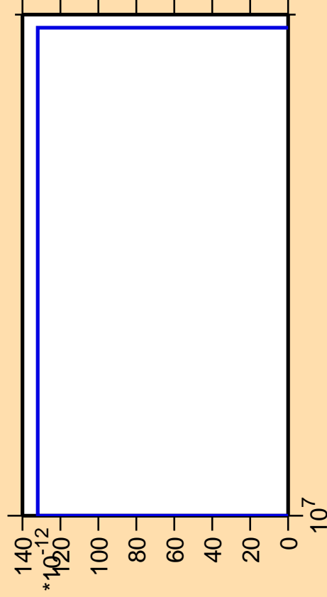
\Delta\sigma/\sigma vs. E for ^{194}\text{Os} (mt 11)
