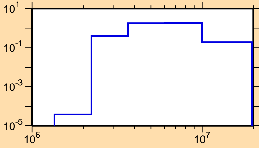
\sigma vs. E for ^{194}\text{Os}(n,n\text{cont.})
