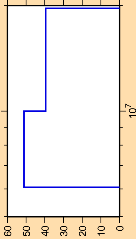
\Delta\sigma/\sigma vs. E for ^{194}\text{Os}(n,p)
