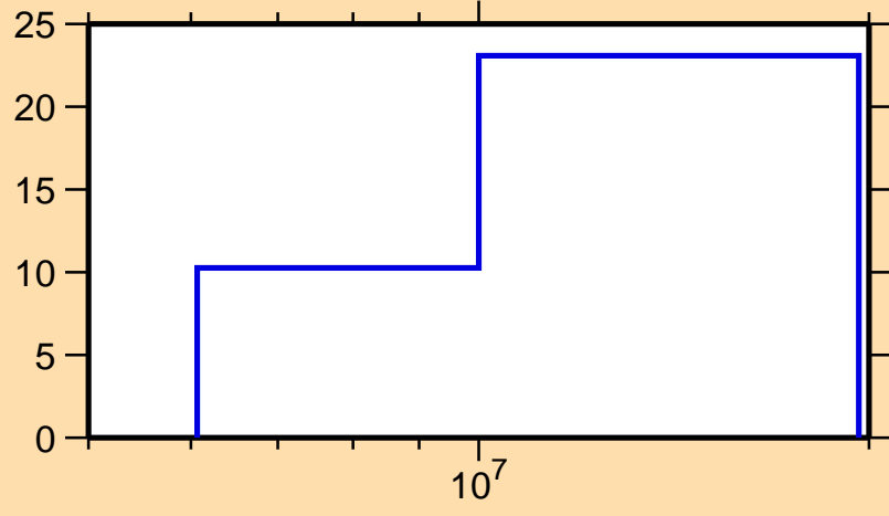
\Delta\sigma/\sigma vs. E for ^{194}\text{Os}(n,n\text{cont.})
