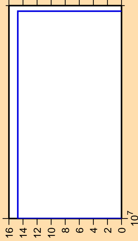
\Delta\sigma/\sigma vs. E for ^{194}\text{Os}(n,3n)
