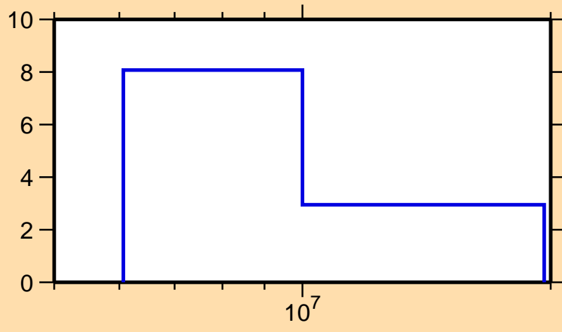
\Delta\sigma/\sigma vs. E for ^{194}\text{Os}(n,\text{el.})
