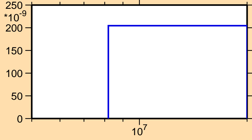
\sigma vs. E for ^{194}\text{Os}(n,n\alpha)
