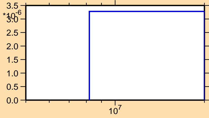
\sigma vs. E for ^{194}\text{Os}(n,np)
