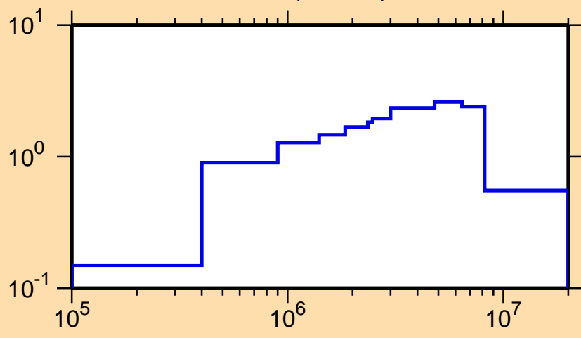
\sigma vs. E for ^{194}\text{Os}(n,\text{inel.})
