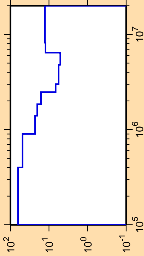
\Delta\sigma/\sigma vs. E for ^{194}\text{Os}(n,\text{inel.})
