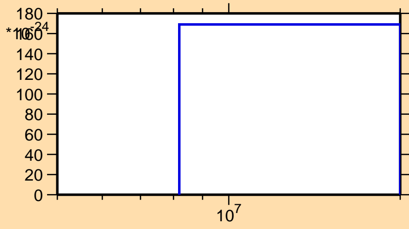
\sigma vs. E for ^{194}\text{Os} (mt 11)
