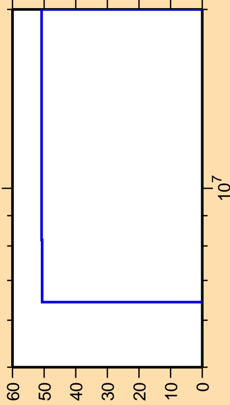
\Delta\sigma/\sigma vs. E for ^{194}\text{Os}(n,\gamma)
