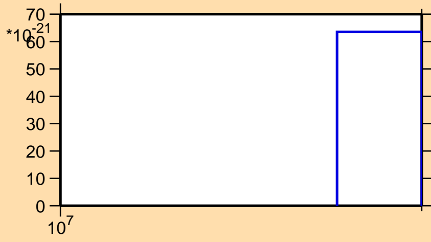
\sigma vs. E for ^{195}\text{Os} (mt 11)
