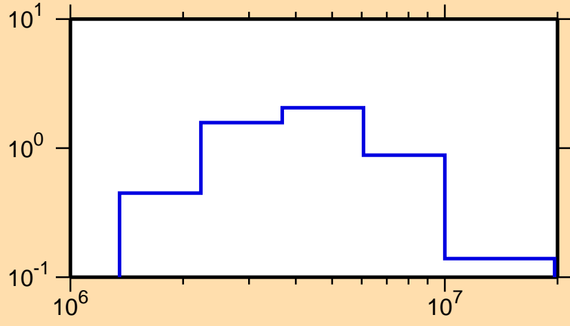
\sigma vs. E for ^{195}\text{Os}(n,n\text{cont.})
