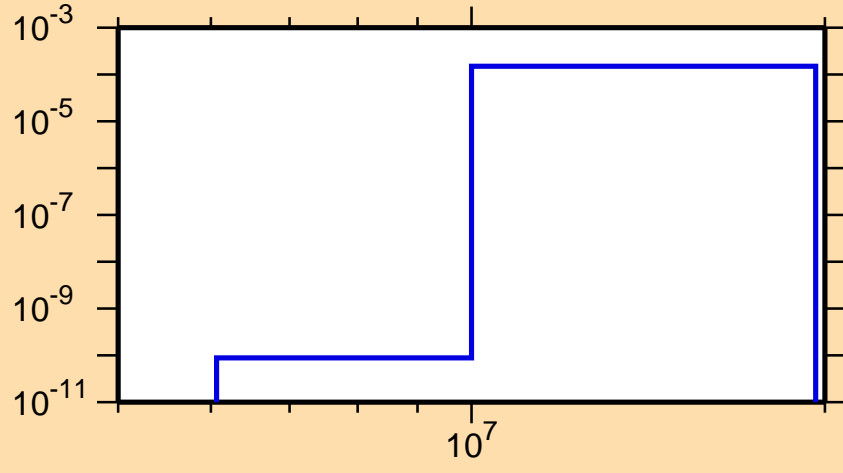
\sigma vs. E for ^{196}\text{Os}(n,p)
