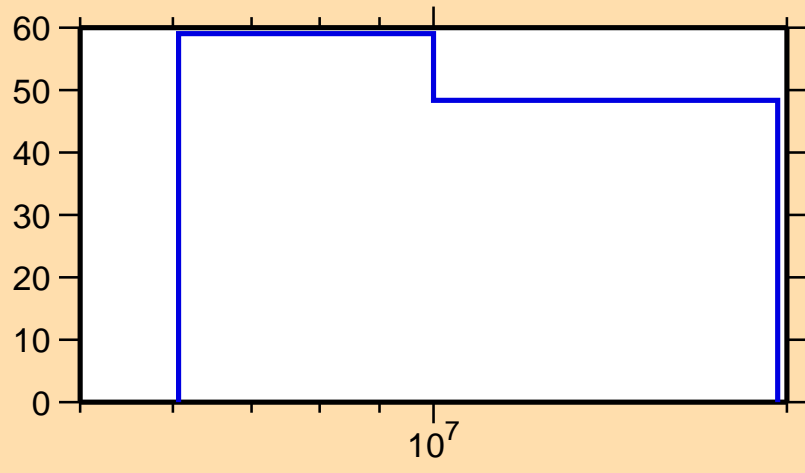
\Delta\sigma/\sigma vs. E for ^{196}\text{Os}(n,n_1)
