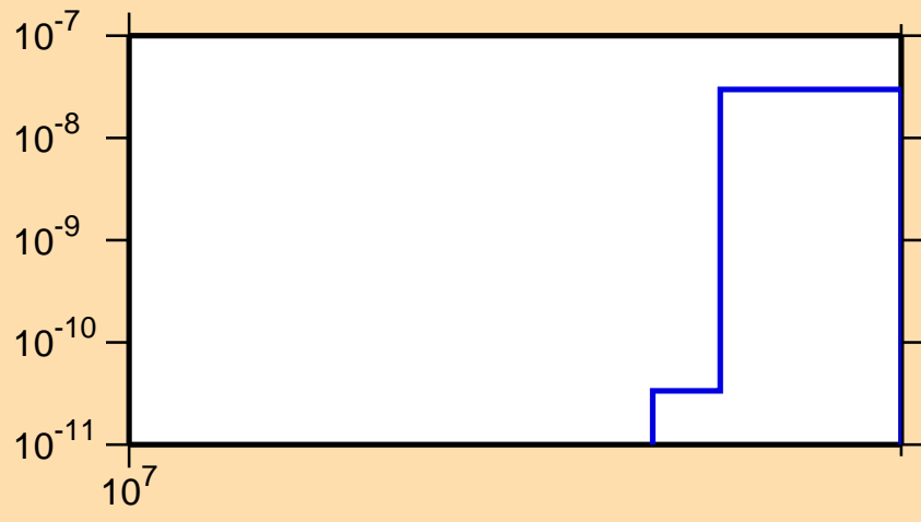
\sigma vs. E for ^{197}\text{Os}(n,\text{nd})
