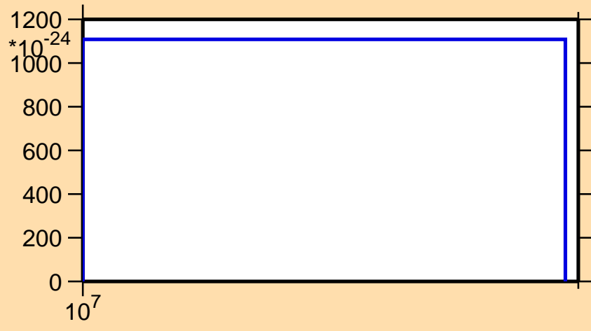
\sigma vs. E for ^{197}\text{Os} (mt 11)
