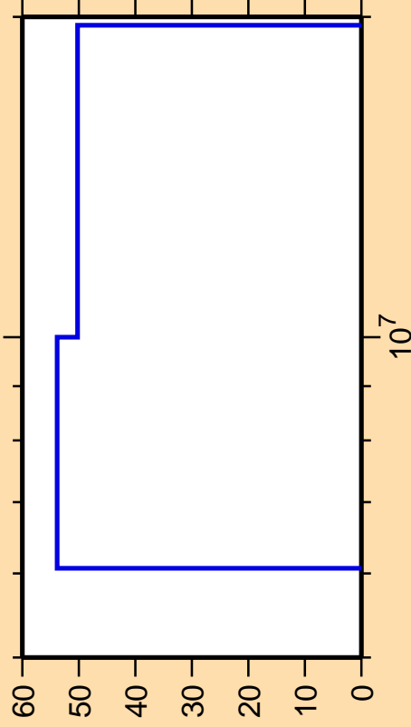
\Delta\sigma/\sigma vs. E for ^{198}\text{Os}(n,n_1)
