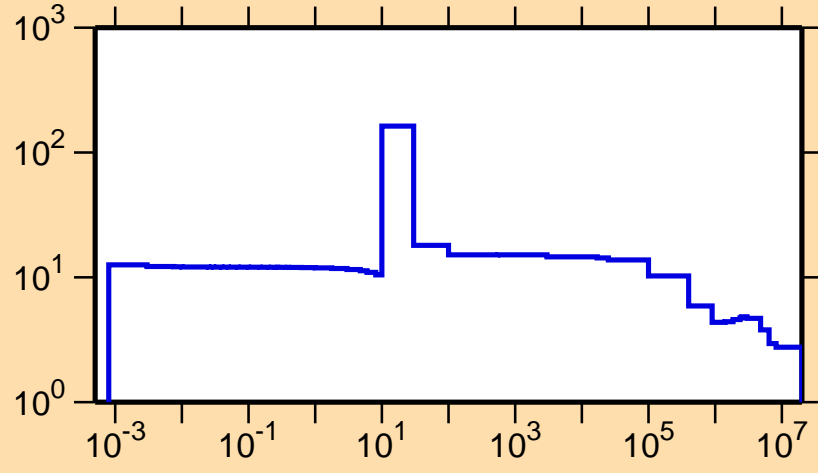
\sigma vs. E for ^{198}\text{Os}(n,\text{el.})
