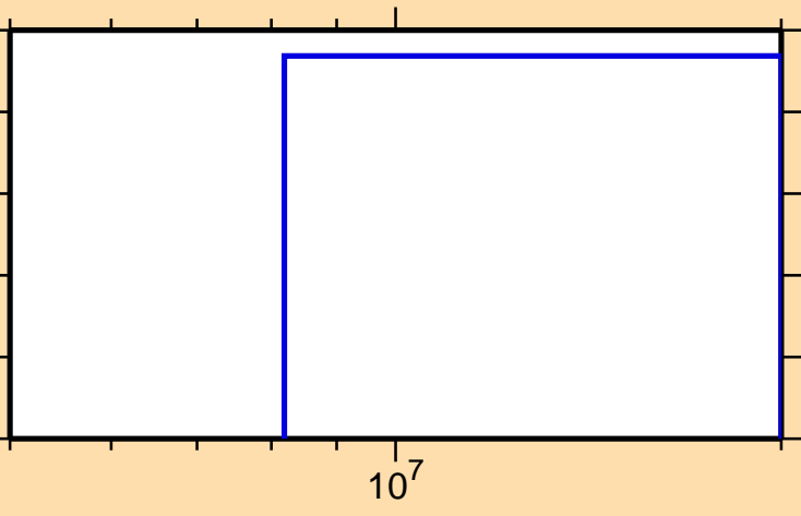
\sigma vs. E for ^{198}\text{Os}(n,2np)
