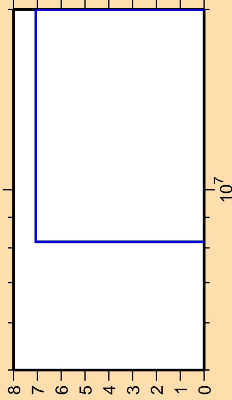
\Delta\sigma/\sigma vs. E for ^{198}\text{Os}(n,nd)
