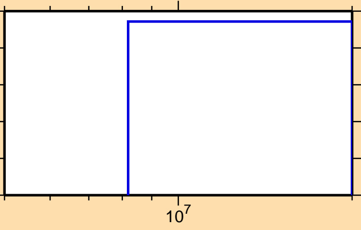
\sigma vs. E for ^{198}\text{Os}(n,d)
