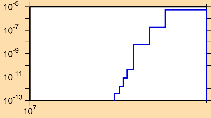
\sigma vs. E for ^{200}\text{Os}(n,np)
