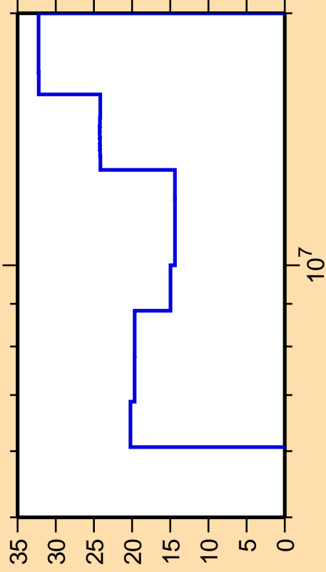
\Delta\sigma/\sigma vs. E for ^{200}\text{Os}(n,2n)
