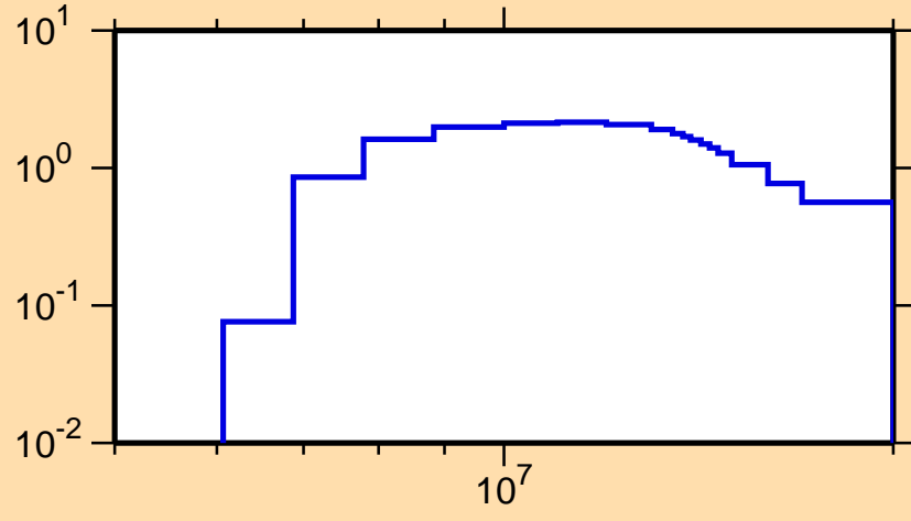
\sigma vs. E for ^{200}\text{Os}(n,2n)
