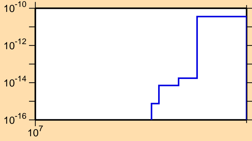
\sigma vs. E for ^{200}\text{Os}(n,\text{nd})
