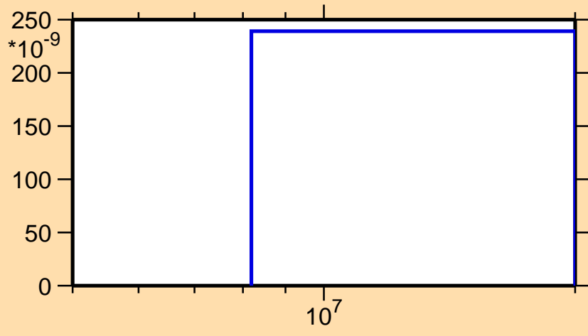
\sigma vs. E for ^{200}\text{Os}(n,\alpha)
