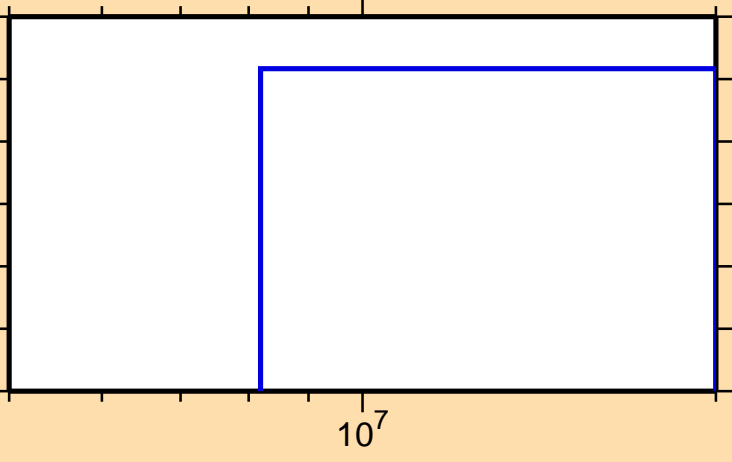
\sigma vs. E for ^{200}\text{Os}(n,n\alpha)
