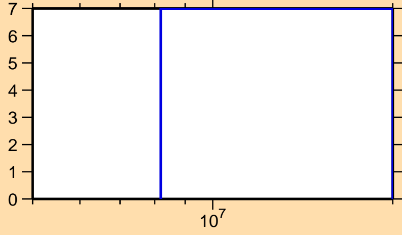
\Delta\sigma/\sigma vs. E for ^{200}\text{Os}(n,\text{el.})
