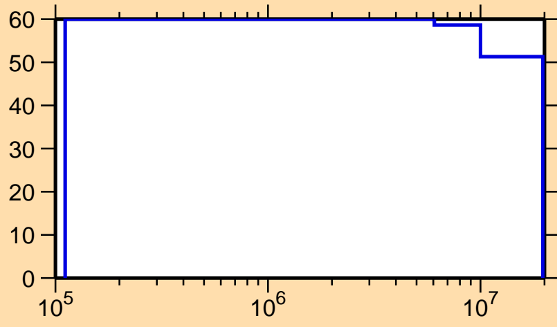
\Delta\sigma/\sigma vs. E for ^{201}\text{Os}(n,n_1)
