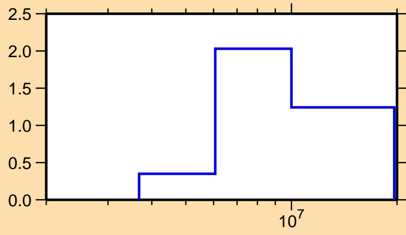
\sigma vs. E for ^{201}\text{Os}(n,2n)
