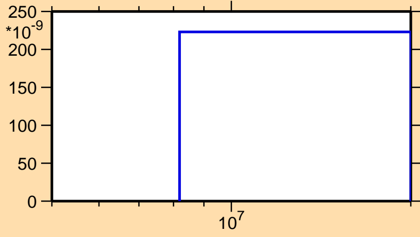
\sigma vs. E for ^{201}\text{Os}(n,\alpha)
