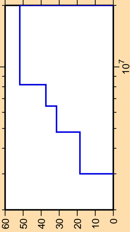
\Delta\sigma/\sigma vs. E for ^{201}\text{Os}(n,n\text{cont.})
