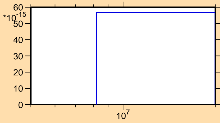
\sigma vs. E for ^{201}\text{Os}(n,2n\alpha)
