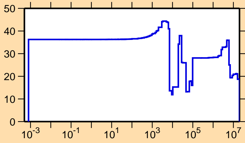
\Delta\sigma/\sigma vs. E for ^{29}\text{P}(n,\gamma)
