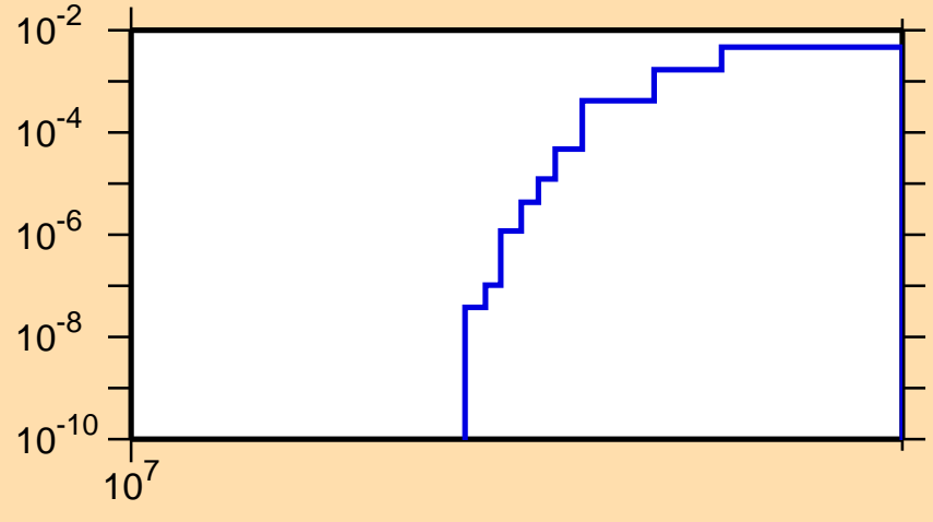
\sigma vs. E for ^{29}\text{P}(n,pd)
