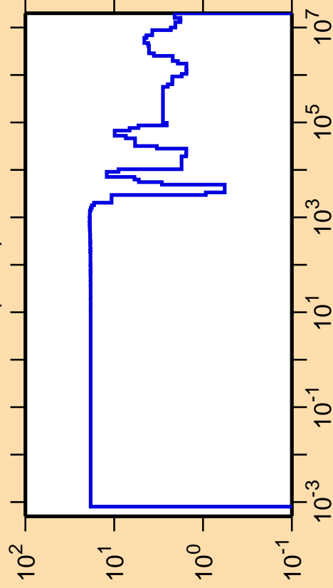
\Delta\sigma/\sigma vs. E for ^{29}\text{P}(n,\text{el.})
