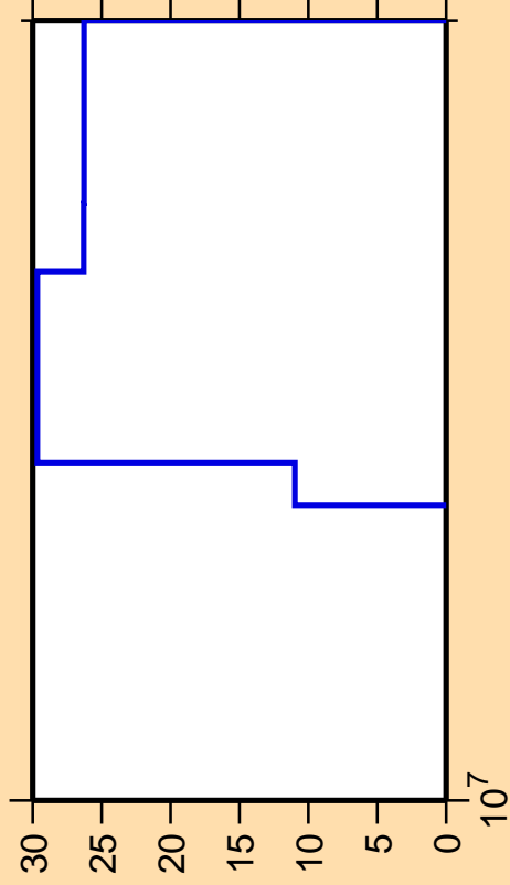
\Delta\sigma/\sigma vs. E for ^{29}\text{P}(n,pd)
