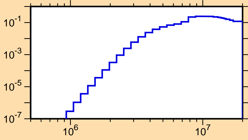
\sigma vs. E for ^{29}\text{P}(n,\alpha)
