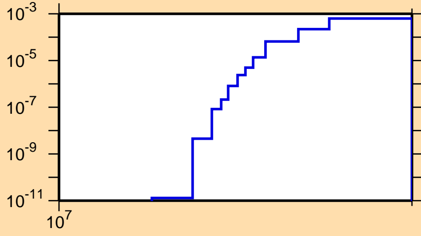
\sigma vs. E for ^{29}\text{P}(\text{mt117})
