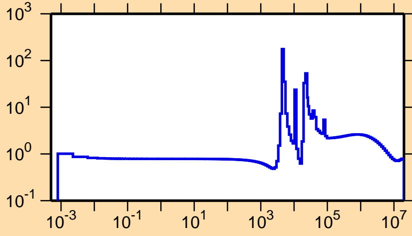
\sigma vs. E for ^{29}\text{P}(n,\text{el.})
