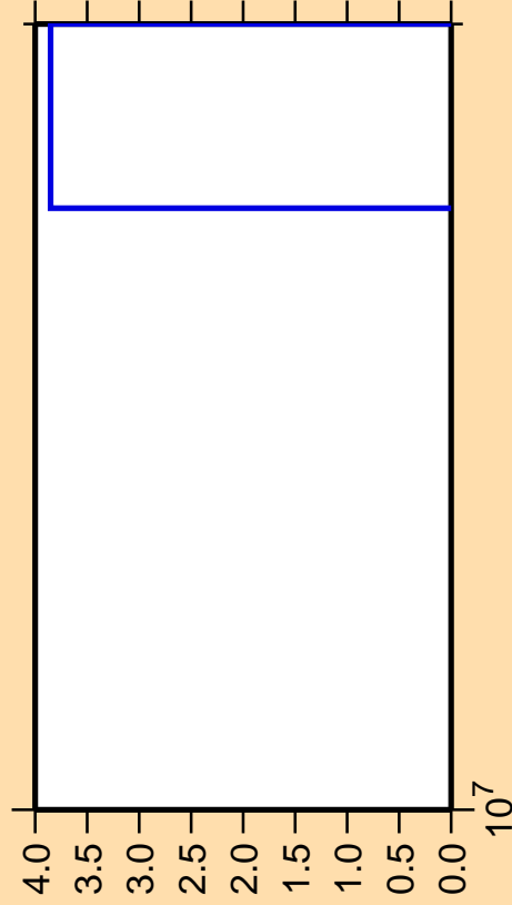
\Delta\sigma/\sigma vs. E for ^{29}\text{P}(n,\text{pt})
