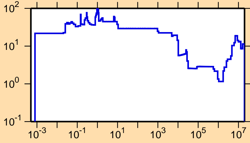
\Delta\sigma/\sigma vs. E for ^{29}\text{P}(n,p)
