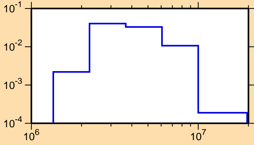
\sigma vs. E for ^{29}\text{P}(n,n_2)
