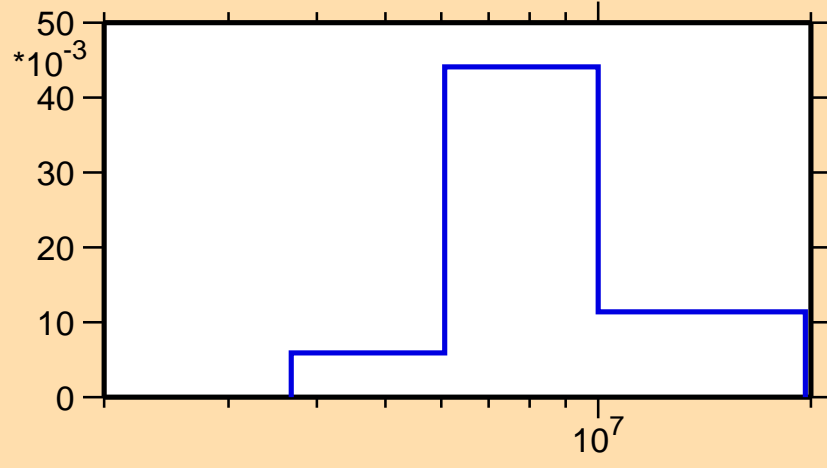
\sigma vs. E for ^{29}\text{P}(n,n\text{cont.})
