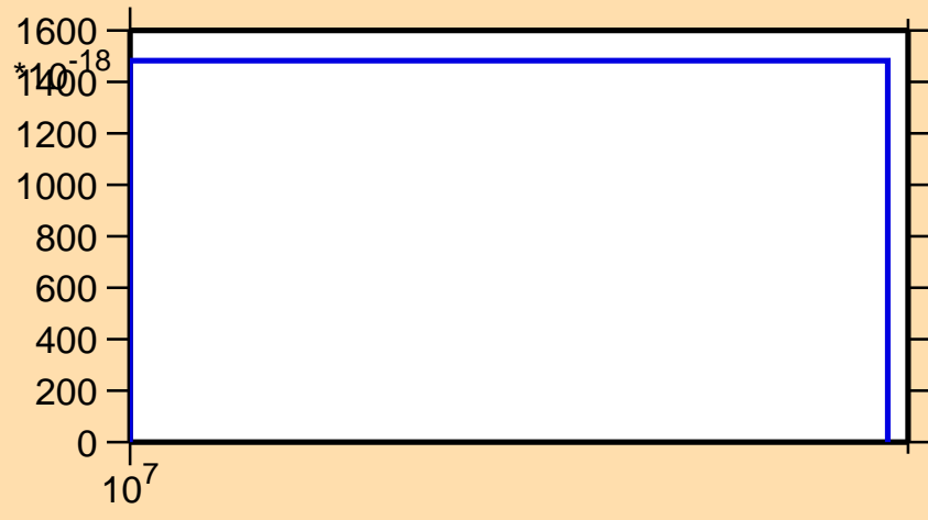
\sigma vs. E for ^{29}\text{P}(n,\text{pt})
