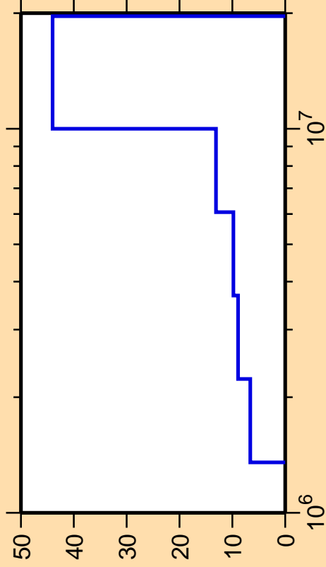
\Delta\sigma/\sigma vs. E for ^{29}\text{P}(n,n_2)
