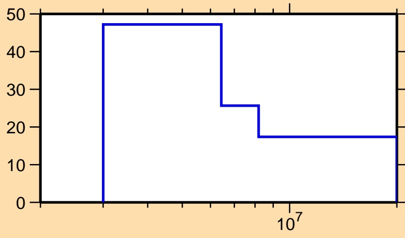
\Delta\sigma/\sigma vs. E for ^{29}\text{P}(n,ncont.)
