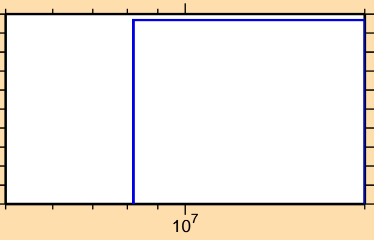
\sigma vs. E for ^{30}\text{P}(\text{mt117})
