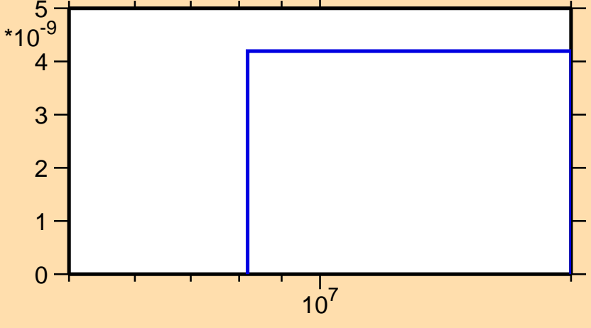
\sigma vs. E for ^{30}\text{P}(n,\text{pd})
