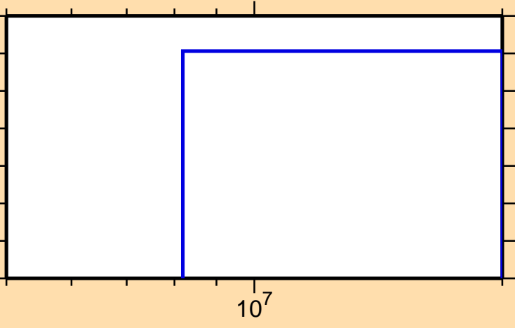
\sigma vs. E for ^{30}\text{P}(n,\text{He}3)
