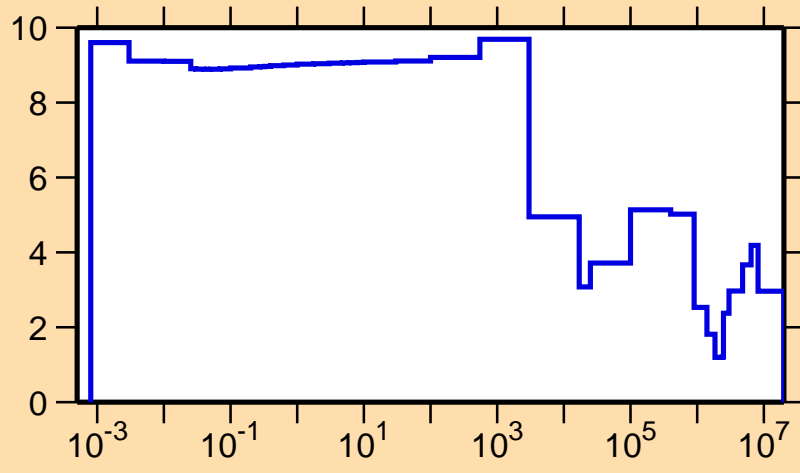
\Delta\sigma/\sigma vs. E for ^{30}\text{P}(n,\text{tot.})
