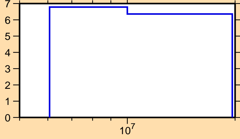
\Delta\sigma/\sigma vs. E for ^{32}\text{P}(n,2n)
