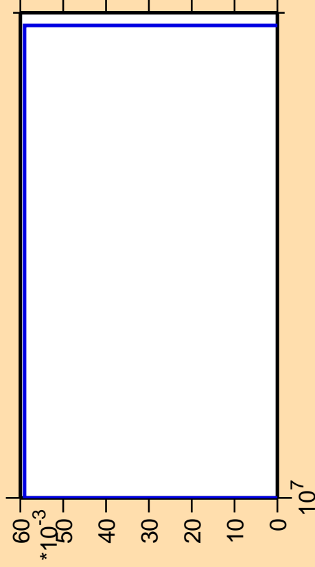
\Delta\sigma/\sigma vs. E for ^{32}\text{P}(n,2n\alpha)
