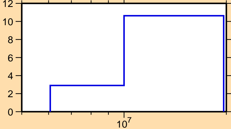
\Delta\sigma/\sigma vs. E for ^{32}\text{P}(n,\text{inel.})
