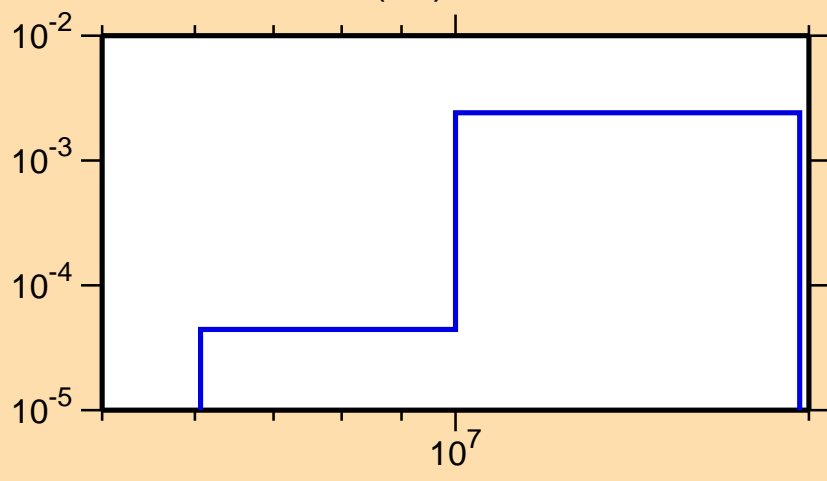
\sigma vs. E for ^{32}\text{P}(n,t)
