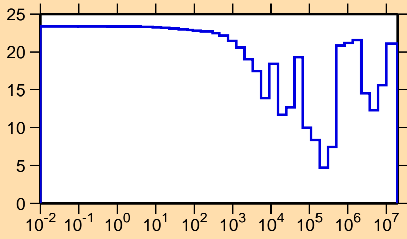
\Delta\sigma/\sigma vs. E for ^{32}\text{P}(n,\gamma)
