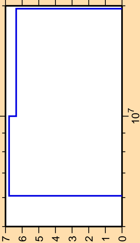
\Delta\sigma/\sigma vs. E for ^{32}\text{P}(n,2n)
