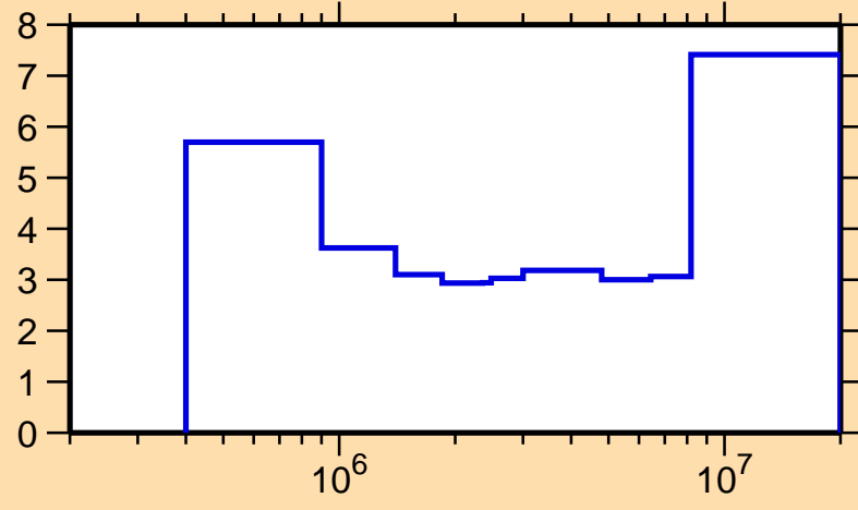
\Delta\sigma/\sigma vs. E for ^{32}\text{P}(n,\text{inel.})
