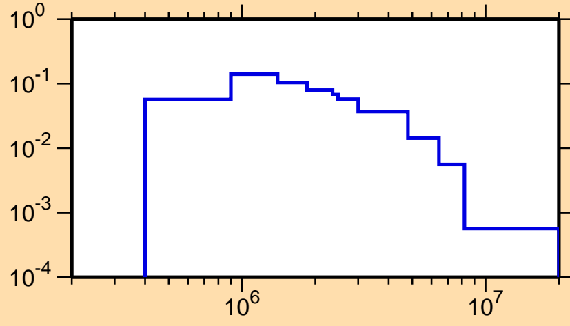
\sigma vs. E for ^{32}\text{P}(n,n_2)
