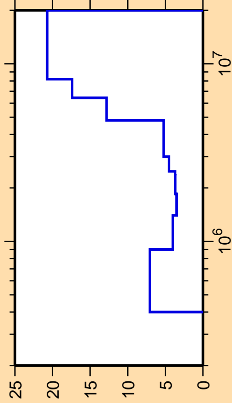
\Delta\sigma/\sigma vs. E for ^{32}\text{P}(n,n_2)
