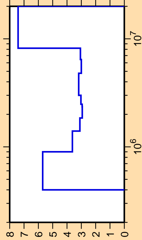
\Delta\sigma/\sigma vs. E for ^{32}\text{P}(n,\text{inel.})
