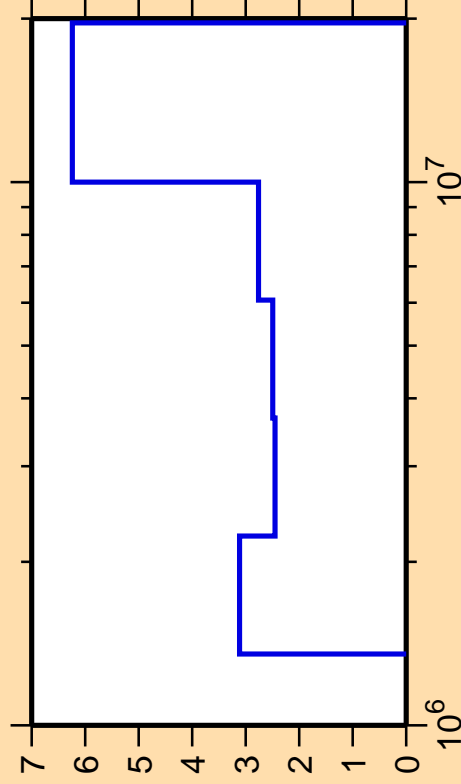
\Delta\sigma/\sigma vs. E for ^{33}\text{P}(n,\text{inel.})
