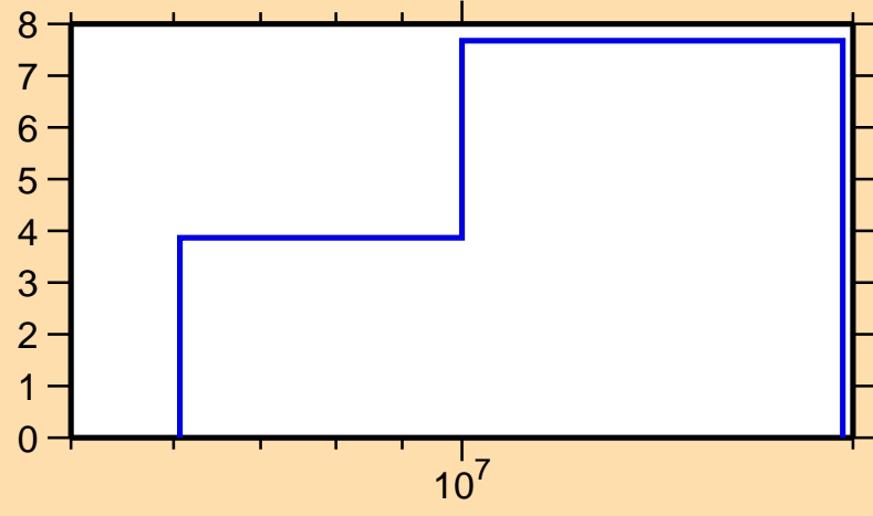
\Delta\sigma/\sigma vs. E for ^{33}\text{P}(n,n\text{cont.})
