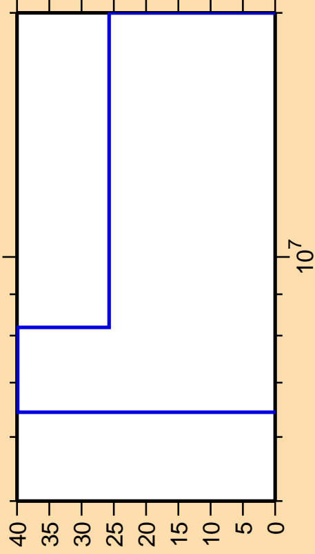
\Delta\sigma/\sigma vs. E for ^{33}\text{P}(n,d)
