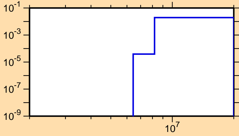
\sigma vs. E for ^{33}\text{P}(n,\alpha)
