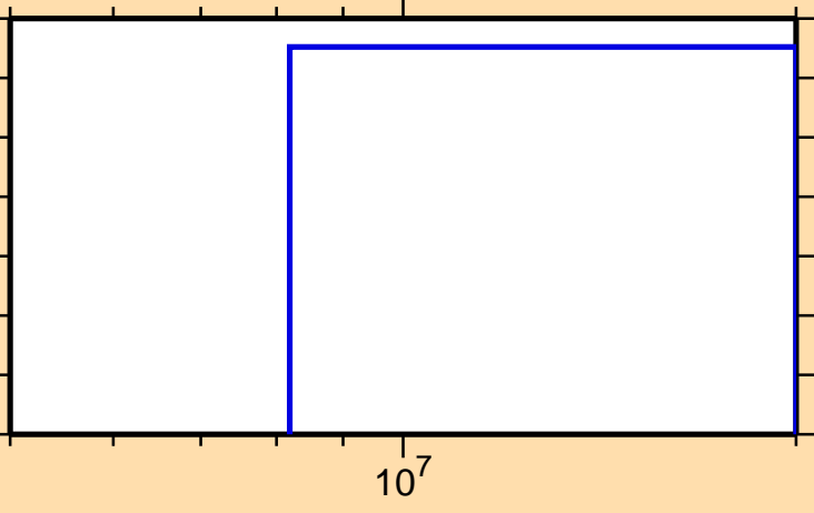
\sigma vs. E for ^{33}\text{P}(n,3n)
