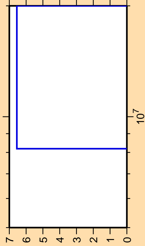
\Delta\sigma/\sigma vs. E for ^{33}\text{P}(n,n\text{cont.})
