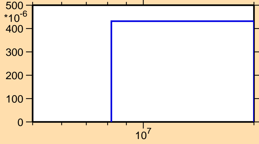
\sigma vs. E for ^{33}\text{P}(n,t)
