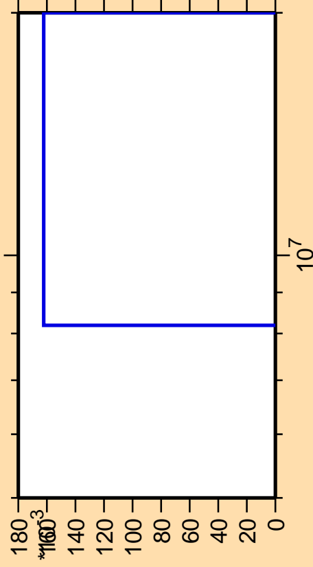
\Delta\sigma/\sigma vs. E for ^{33}\text{P}(n,2np)
