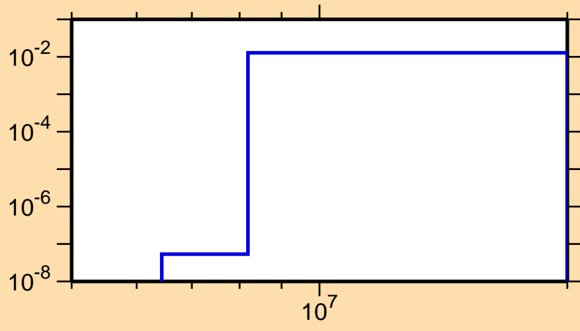
\sigma vs. E for ^{33}\text{P}(n,d)
