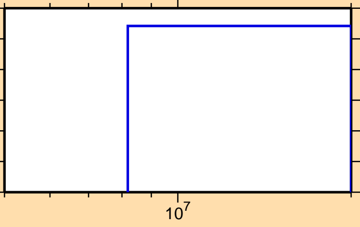
\sigma vs. E for ^{33}\text{P}(n,n\alpha)
