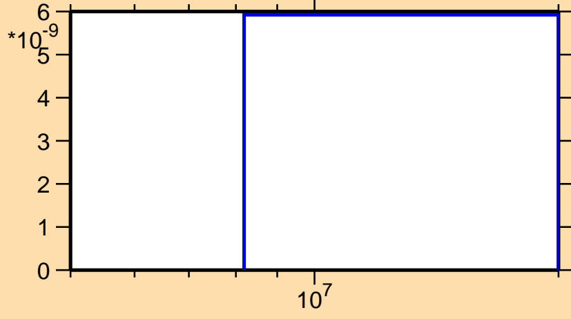
\sigma vs. E for ^{33}\text{P}(n,nt)
