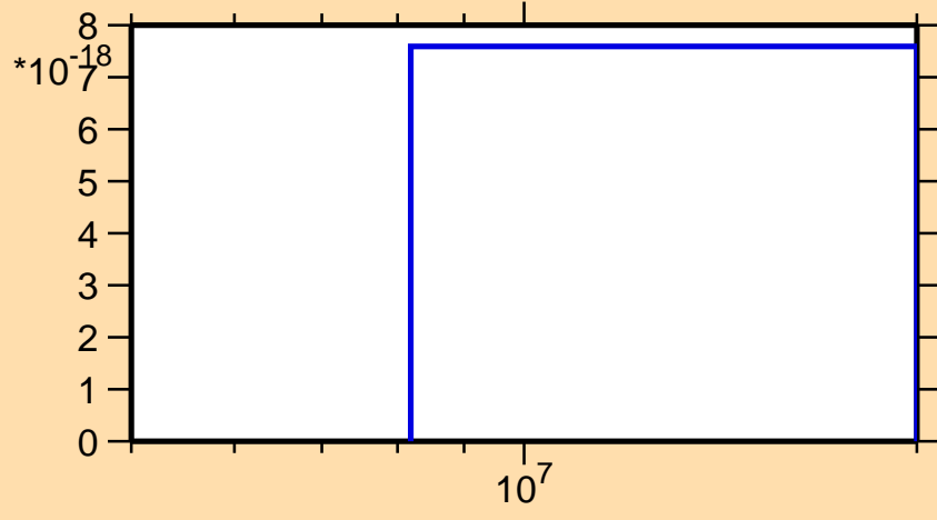
\sigma vs. E for ^{33}\text{P}(n,\text{He}3)
