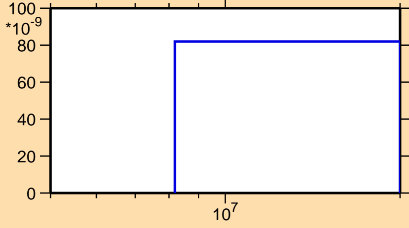
\sigma vs. E for ^{33}\text{P}(n,nd)
