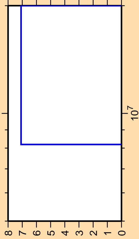
\Delta\sigma/\sigma vs. E for ^{33}\text{P}(n,np)
