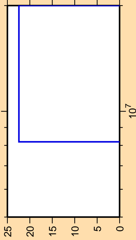
\Delta\sigma/\sigma vs. E for ^{33}\text{P}(n,p)
