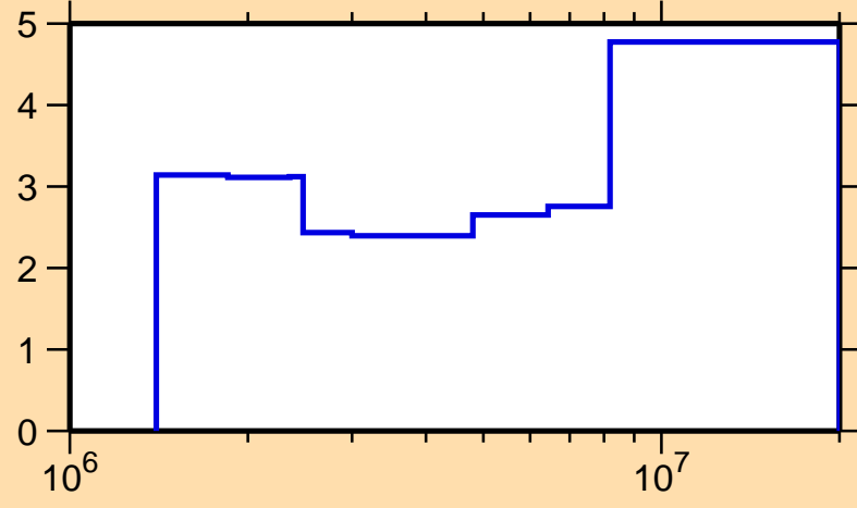
\Delta\sigma/\sigma vs. E for ^{33}\text{P}(n,\text{inel.})
