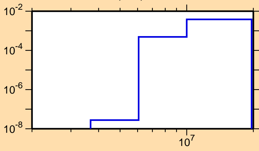
\sigma vs. E for ^{34}\text{P}(n,\alpha)
