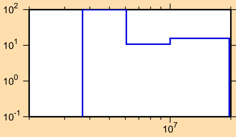
\Delta\sigma/\sigma vs. E for ^{34}\text{P}(n,n\text{cont.})
