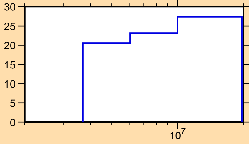
\Delta\sigma/\sigma vs. E for ^{34}\text{P}(n,p)
