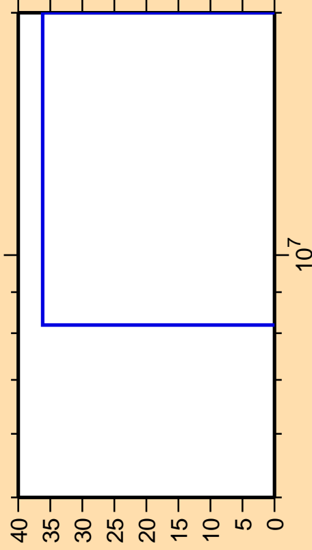
\Delta\sigma/\sigma vs. E for ^{34}\text{P}(n,\text{nd})
