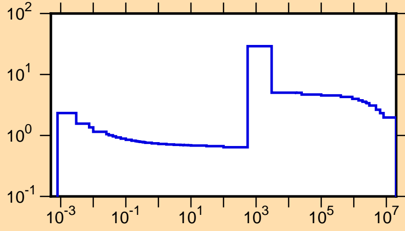
\sigma vs. E for ^{34}\text{P}(n,\text{tot.})
