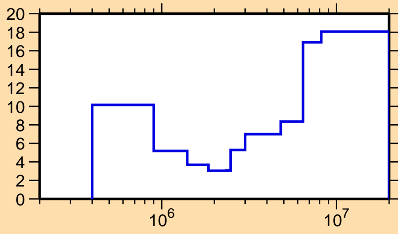
\Delta\sigma/\sigma vs. E for ^{34}\text{P}(n,n_1)
