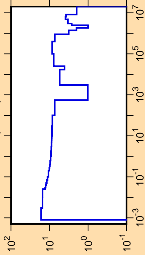
\Delta\sigma/\sigma vs. E for ^{34}\text{P}(n,\text{tot.})
