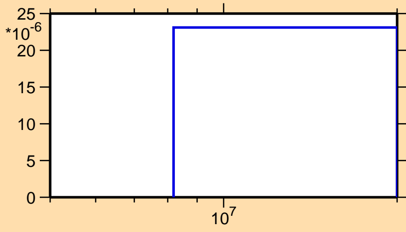
\sigma vs. E for ^{34}\text{P}(n,\text{nd})
