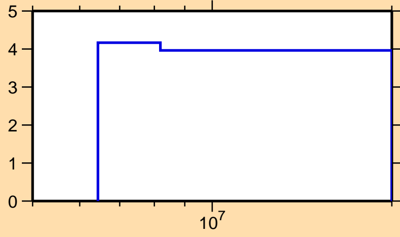
\Delta\sigma/\sigma vs. E for ^{34}\text{P}(n,2n)
