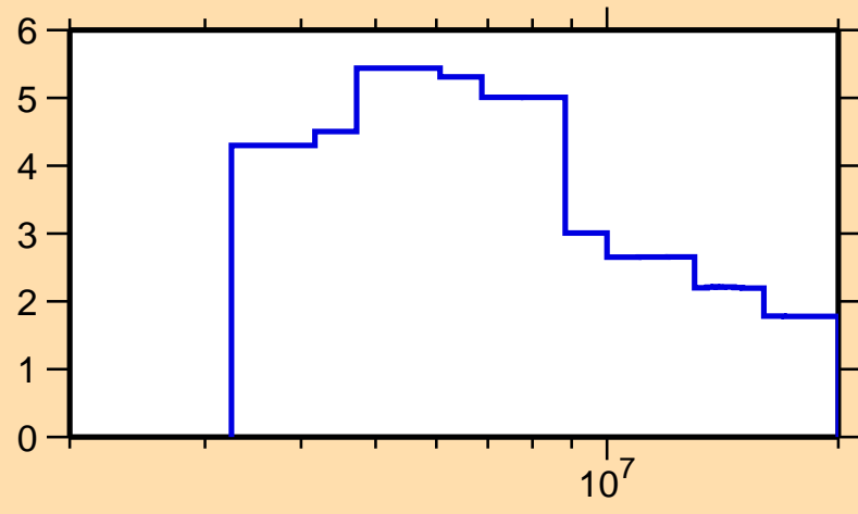
\Delta\sigma/\sigma vs. E for ^{36}\text{P}(n,\text{tot.})
