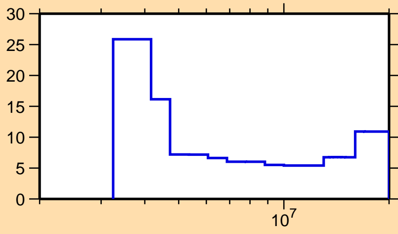
\Delta\sigma/\sigma vs. E for ^{36}\text{P}(n,2n)
