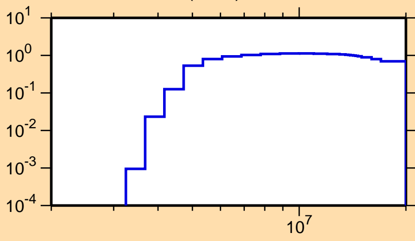
\sigma vs. E for ^{36}\text{P}(n,2n)
