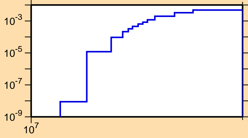
\sigma vs. E for ^{36}\text{P}(n,d)
