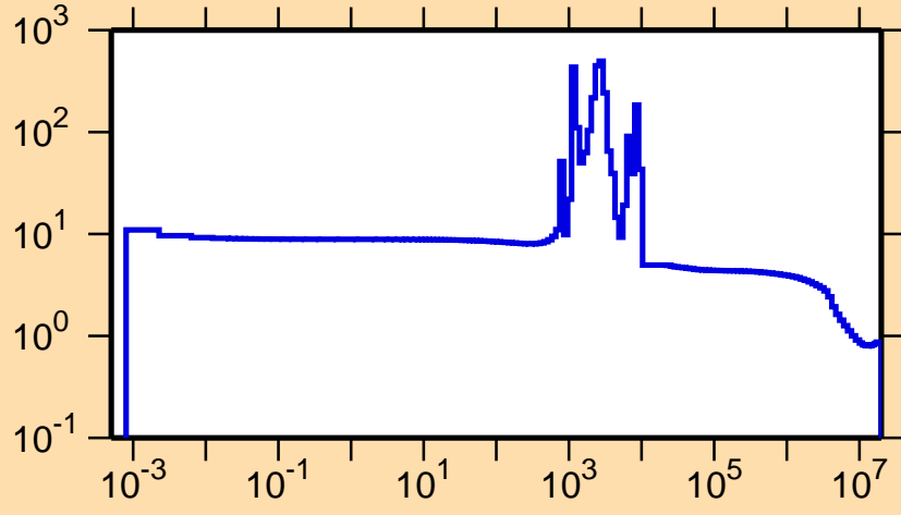
\sigma vs. E for ^{36}\text{P}(n,\text{el.})
