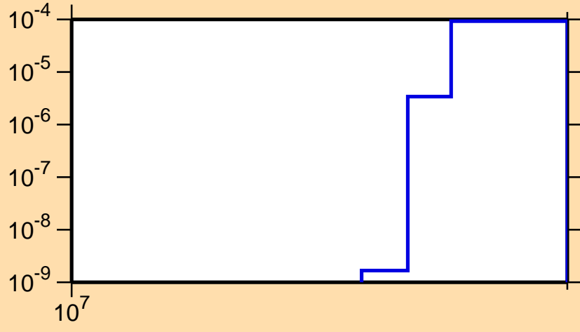
\sigma vs. E for ^{36}\text{P}(n,nt)
