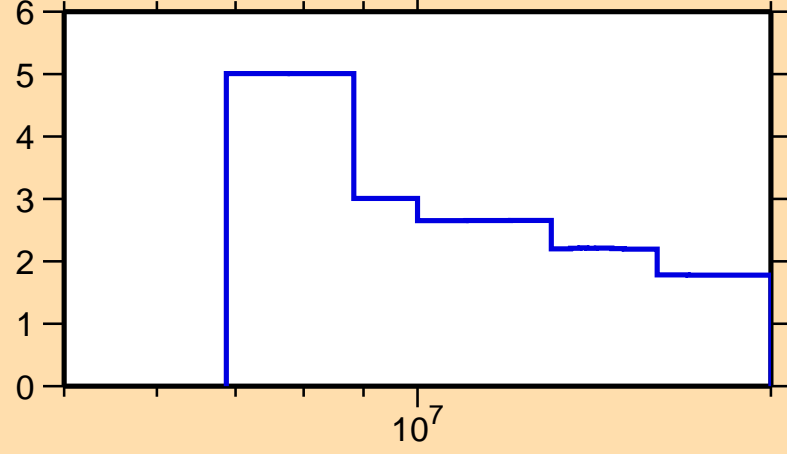
\Delta\sigma/\sigma vs. E for ^{36}\text{P}(n,\text{tot.})
