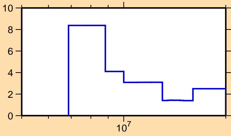
\Delta\sigma/\sigma vs. E for ^{36}\text{P}(n,el.)
