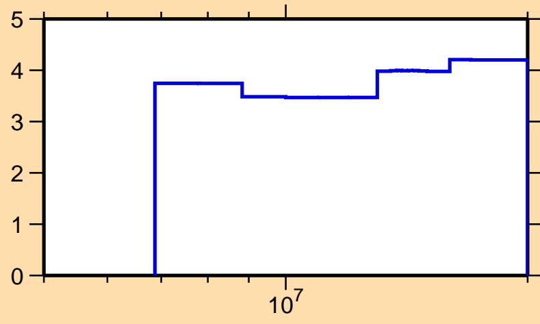
\Delta\sigma/\sigma vs. E for ^{36}\text{P}(n,\text{nonel.})
