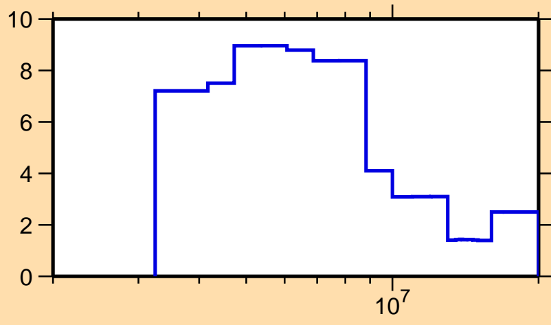
\Delta\sigma/\sigma vs. E for ^{36}\text{P}(n,\text{el.})
