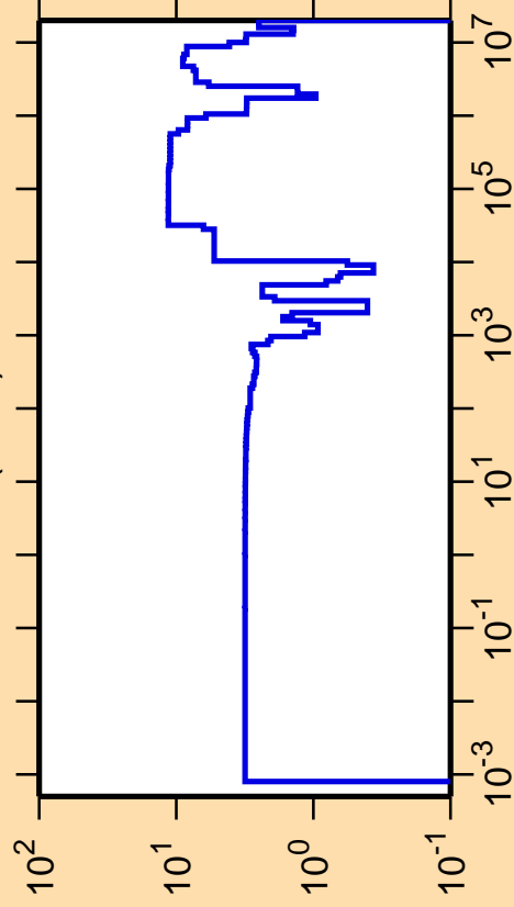
\Delta\sigma/\sigma vs. E for ^{36}\text{P}(n,\text{el.})
