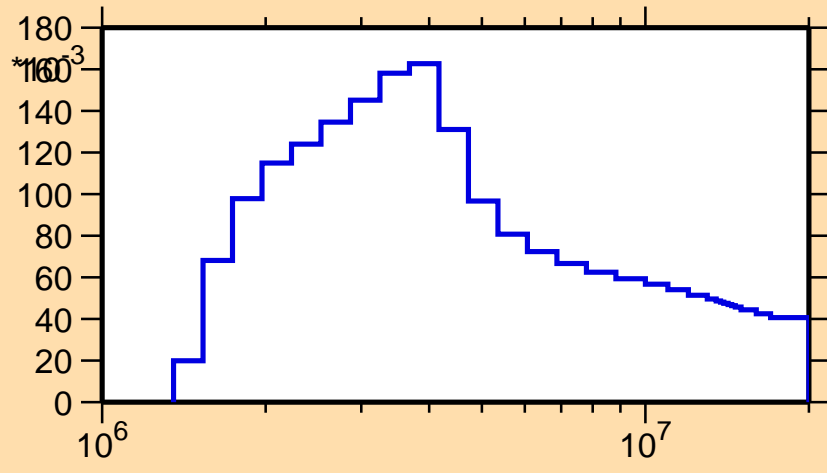
\sigma vs. E for ^{36}\text{P}(n,n_4)
