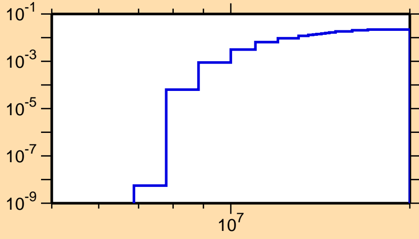
\sigma vs. E for ^{36}\text{P}(n,p)
