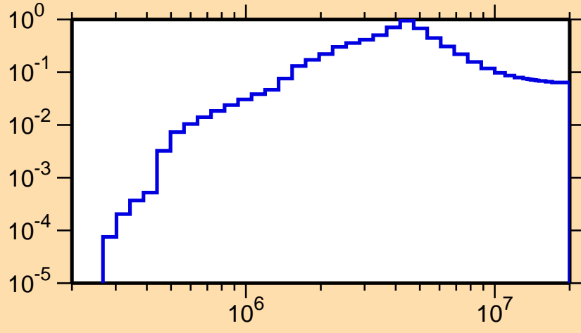
\sigma vs. E for ^{36}\text{P}(n,\text{inel.})
