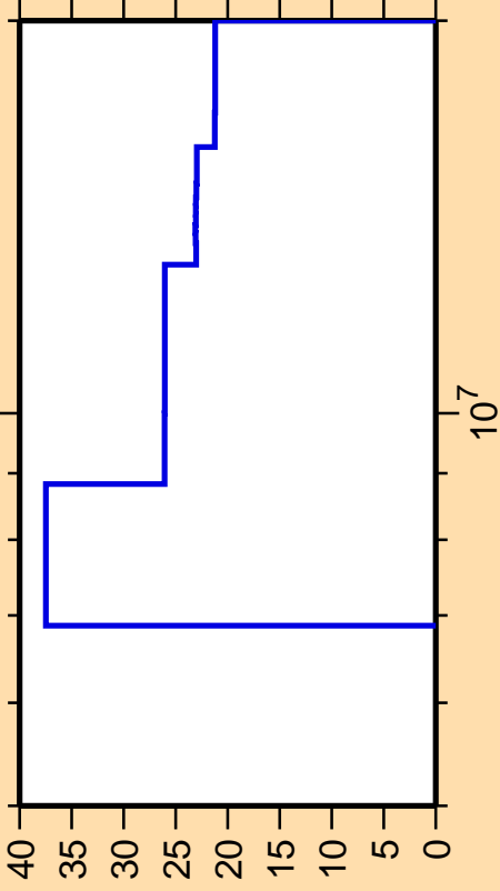
\Delta\sigma/\sigma vs. E for ^{36}\text{P}(n,p)
