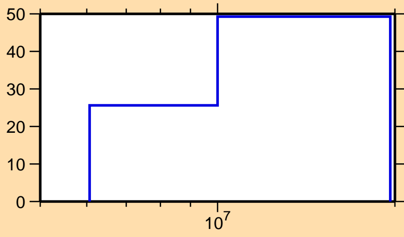
\Delta\sigma/\sigma vs. E for ^{36}\text{P}(n,n_1)
