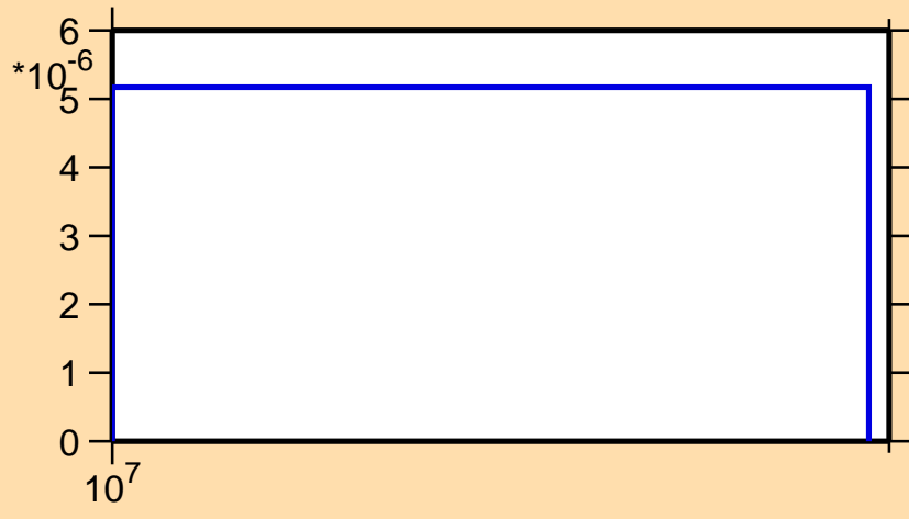
\sigma vs. E for ^{36}\text{P}(n,nd)
