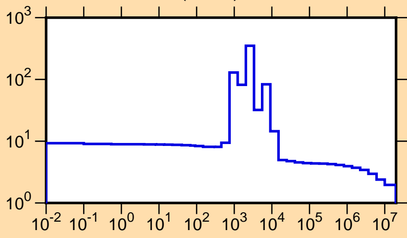
\sigma vs. E for ^{36}\text{P}(n,\text{tot.})
