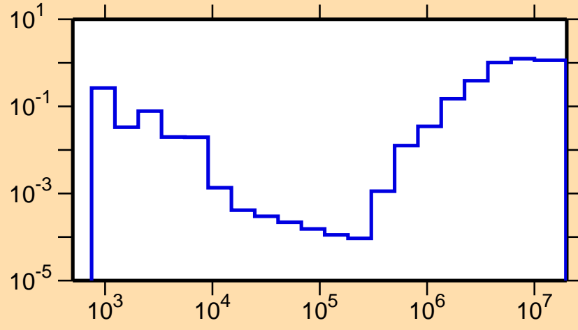
\sigma vs. E for ^{36}\text{P}(n,\text{nonel.})
