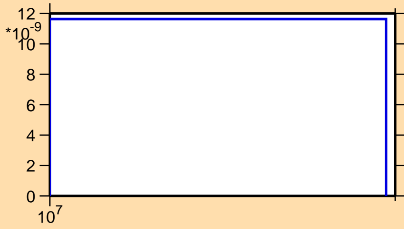
\sigma vs. E for ^{36}\text{P}(n,2np)
