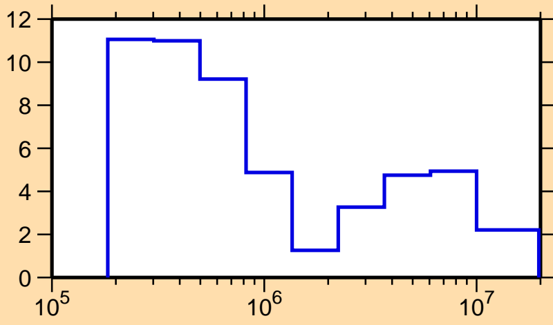
\Delta\sigma/\sigma vs. E for ^{36}\text{P}(n,\text{tot.})
