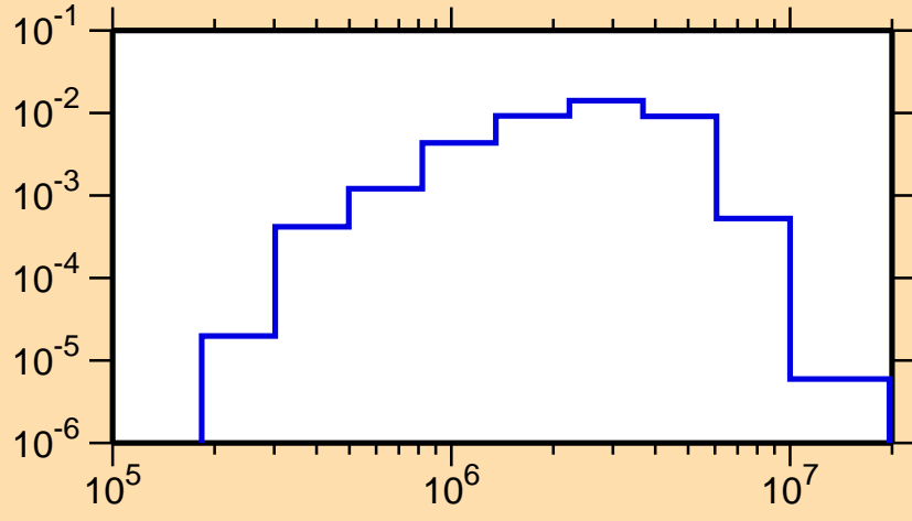
\sigma vs. E for ^{36}\text{P}(n,n_1)
