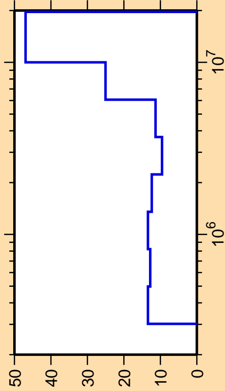
\Delta\sigma/\sigma vs. E for ^{36}\text{P}(n,n_2)
