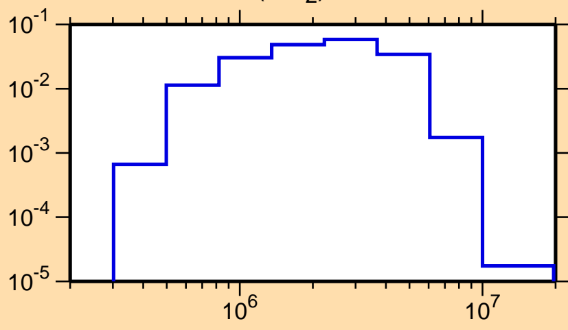
\sigma vs. E for ^{36}\text{P}(n,n_2)
