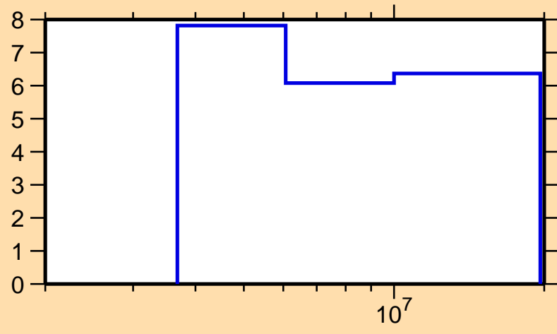
\Delta\sigma/\sigma vs. E for ^{36}\text{P}(n,2n)
