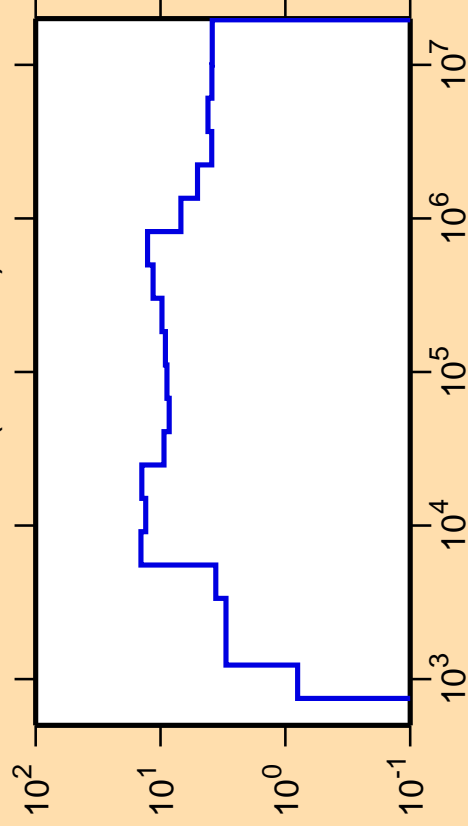
\Delta\sigma/\sigma vs. E for ^{36}\text{P}(n,\text{nonel.})
