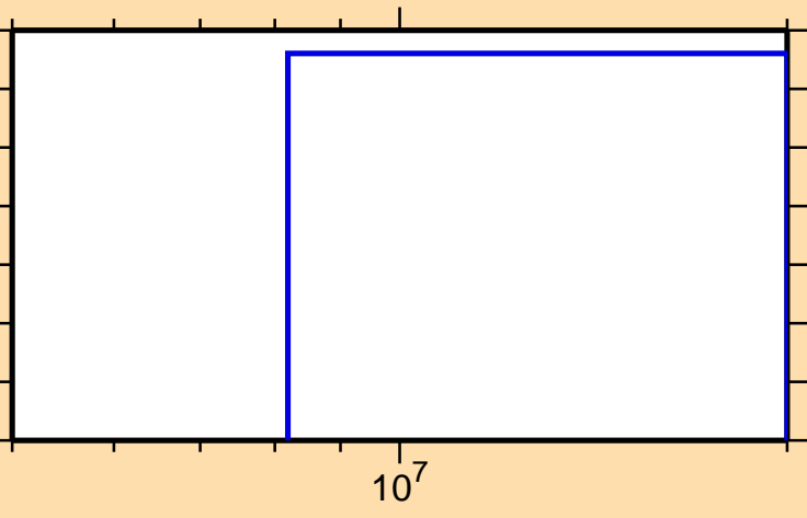
\sigma vs. E for ^{36}\text{P}(n,2np)
