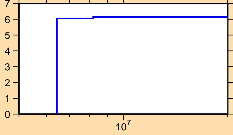
\Delta\sigma/\sigma vs. E for ^{36}\text{P}(n,2n)
