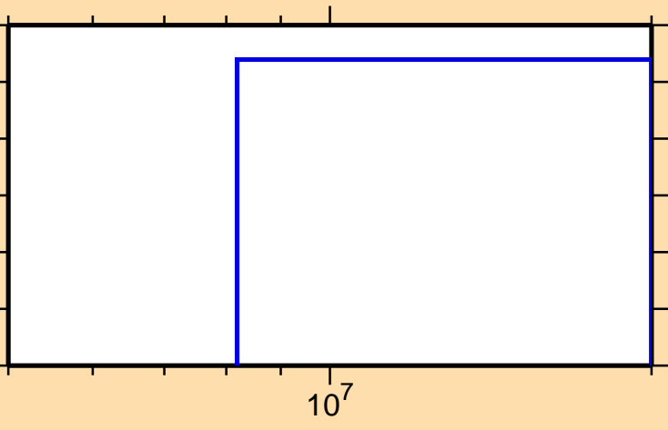
\sigma vs. E for ^{36}\text{P}(n,np)
