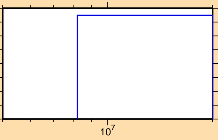
\sigma vs. E for ^{36}\text{P}(n,n\alpha)
