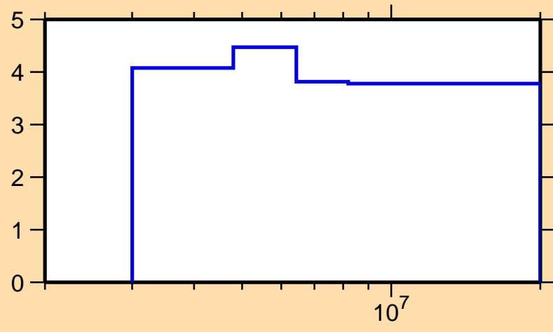
\Delta\sigma/\sigma vs. E for ^{36}\text{P}(n,n\text{onel.})
