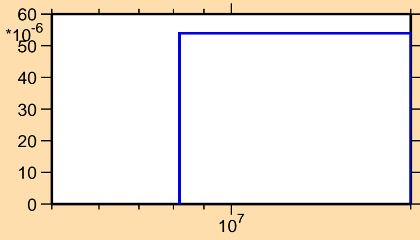
\sigma vs. E for ^{36}\text{P}(n,np)
