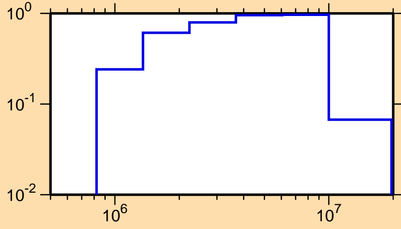
\sigma vs. E for ^{37}\text{P}(n,\text{inel.})
