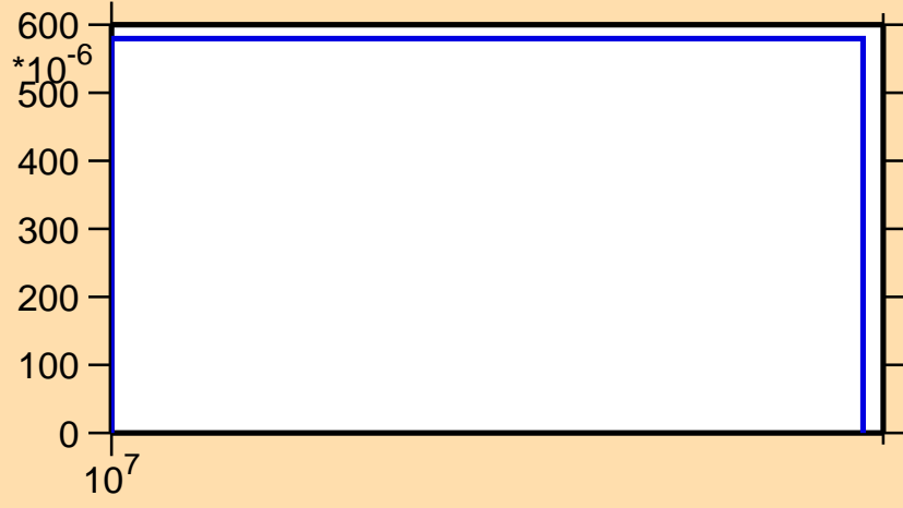
\sigma vs. E for ^{37}\text{P}(n,d)
