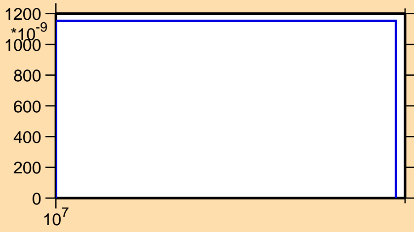
\sigma vs. E for ^{37}\text{P}(n,np)
