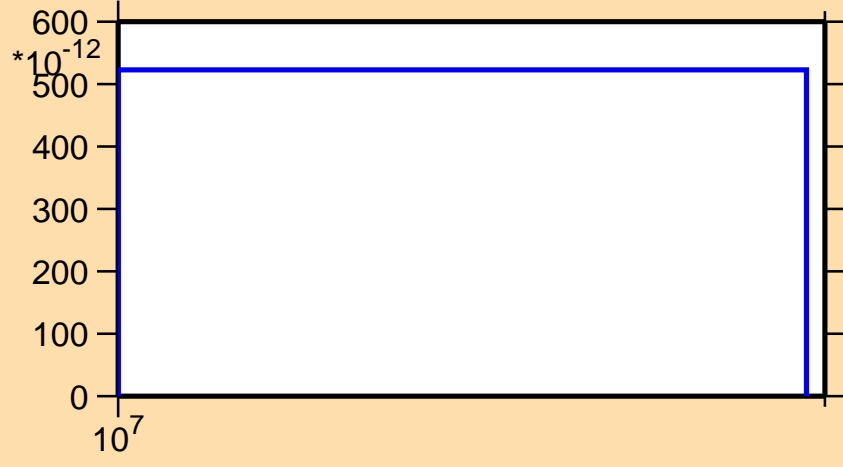
\sigma vs. E for ^{37}\text{P}(n,nd)
