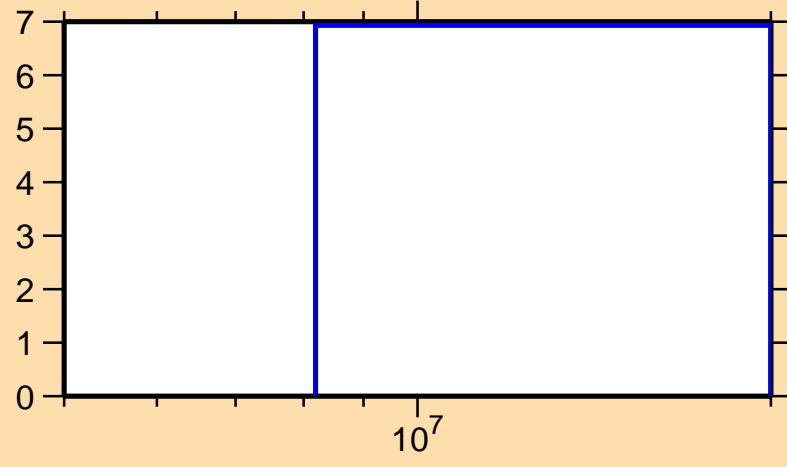
\Delta\sigma/\sigma vs. E for ^{37}\text{P}(n,n\text{onel.})
