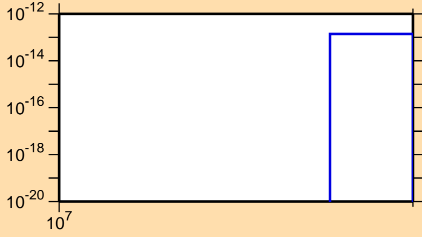
\sigma vs. E for ^{225}\text{Pa} (mt 42)
