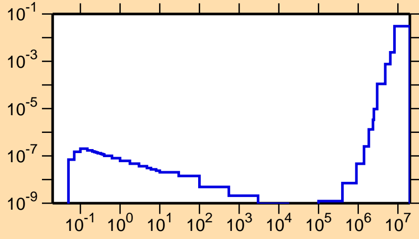
\sigma vs. E for ^{225}\text{Pa}(n,p)
