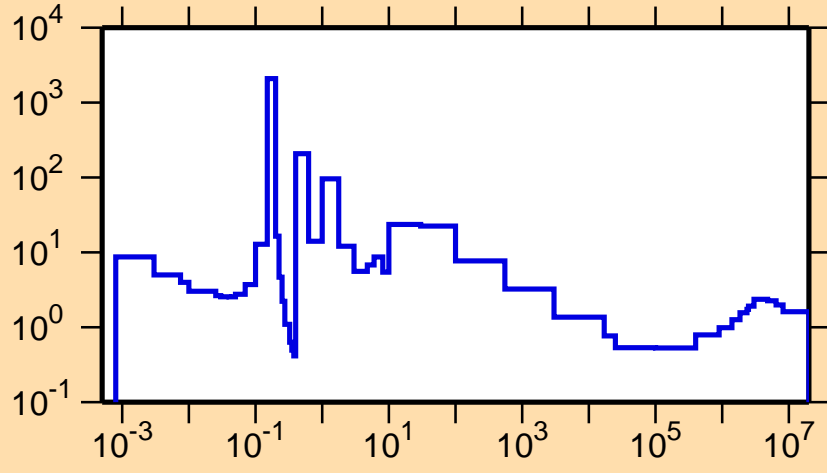
\sigma vs. E for ^{225}\text{Pa}(n,f)
