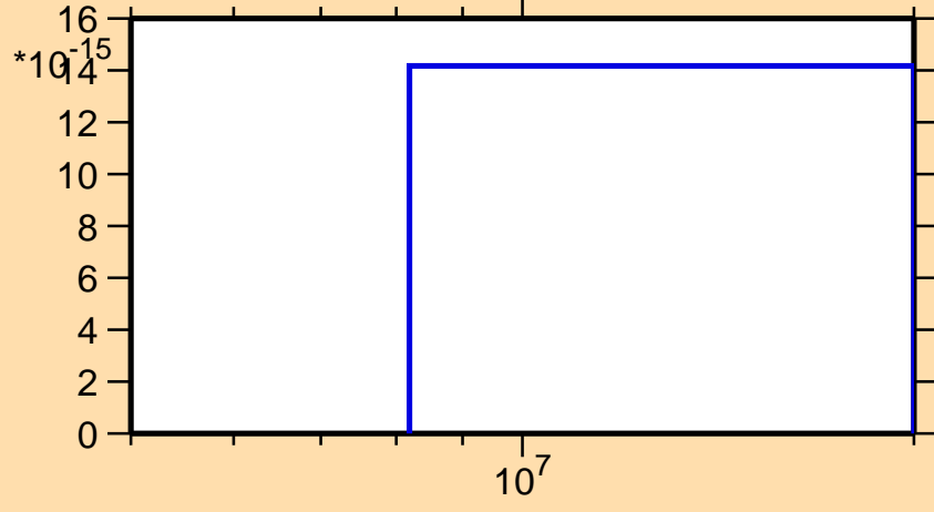
\sigma vs. E for ^{225}\text{Pa}(\text{mt } 34)
