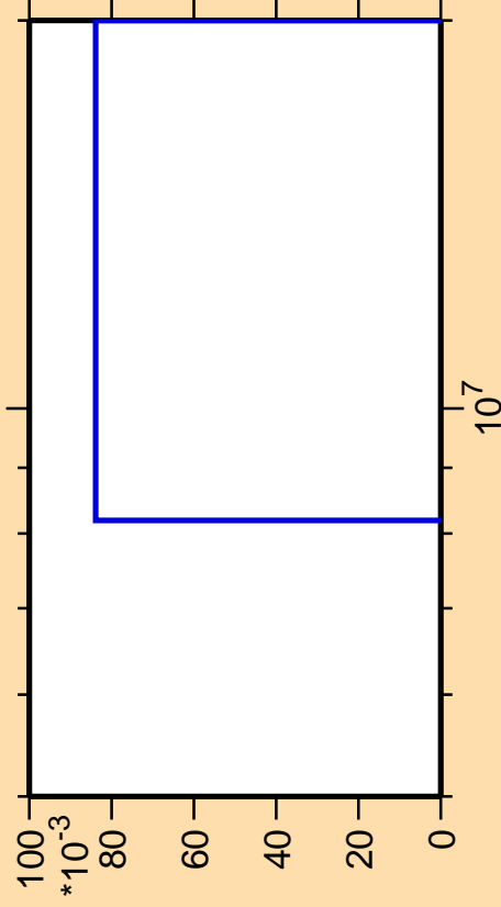
\Delta\sigma/\sigma vs. E for ^{225}\text{Pa}(\text{mt } 34)
