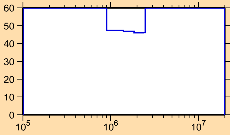
\Delta\sigma/\sigma vs. E for ^{225}\text{Pa}(n,f)
