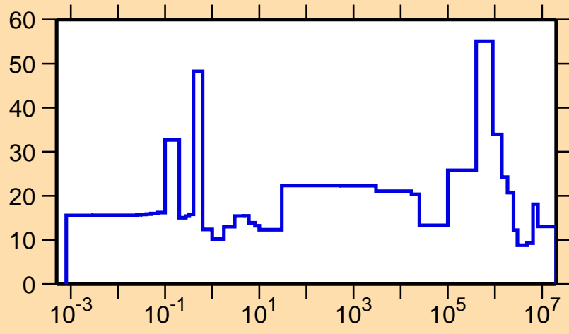
\Delta\sigma/\sigma vs. E for ^{225}\text{Pa}(n,el.)
