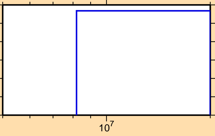
\sigma vs. E for ^{225}\text{Pa} (mt 42)
