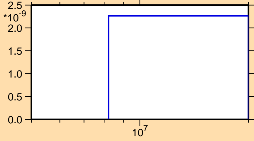
\sigma vs. E for ^{225}\text{Pa} (mt 45)
