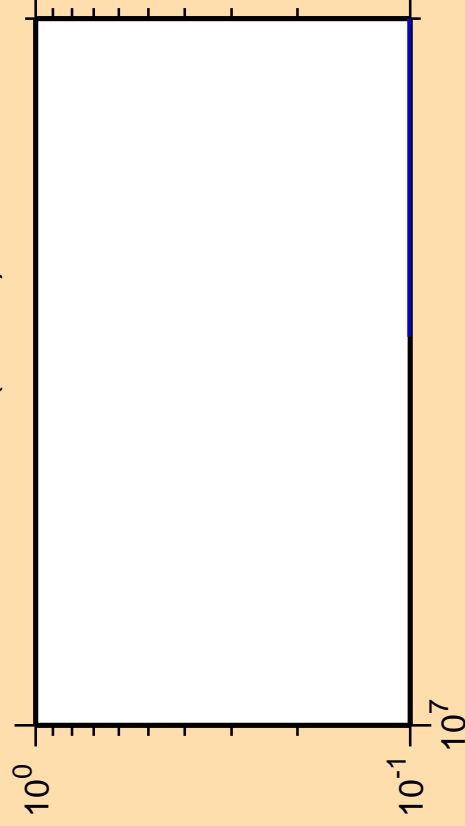
\Delta\sigma/\sigma vs. E for ^{226}\text{Pa}(\text{mt } 11)
