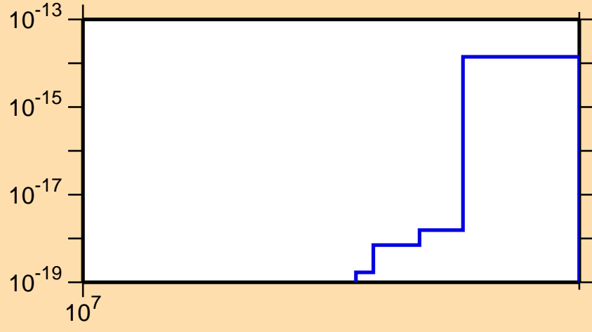
\sigma vs. E for ^{226}\text{Pa}(\text{mt } 11)
