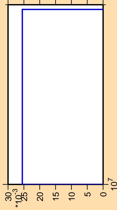
\Delta\sigma/\sigma vs. E for ^{226}\text{Pa} (mt 34)
