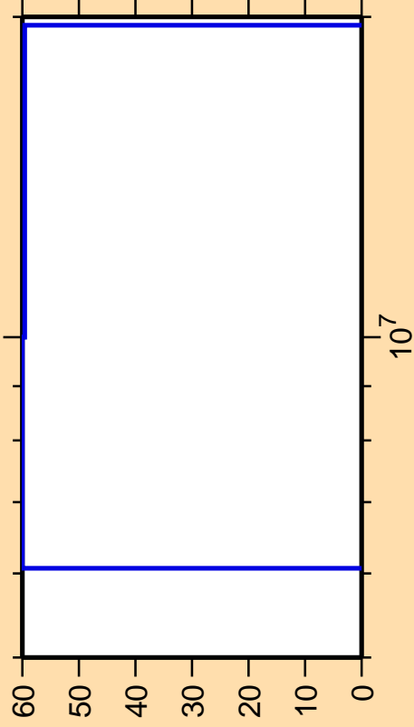
\Delta\sigma/\sigma vs. E for ^{226}\text{Pa}(n,2n)
