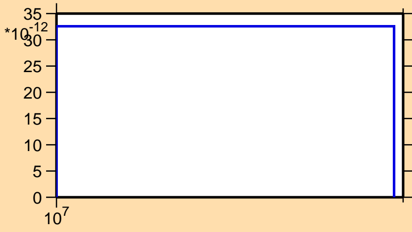
\sigma vs. E for ^{226}\text{Pa} (mt 45)
