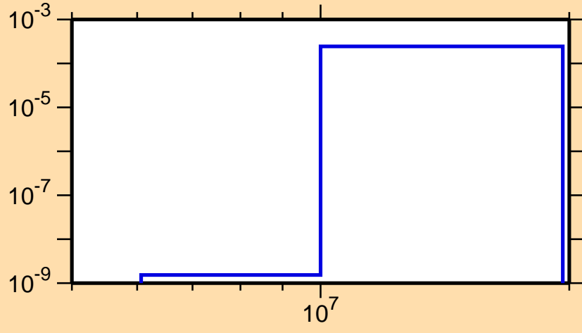
\sigma vs. E for ^{226}\text{Pa}(n,t)
