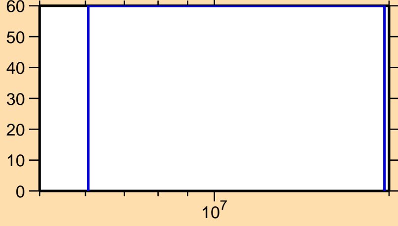
\Delta\sigma/\sigma vs. E for ^{226}\text{Pa}(n,\text{inel.})
