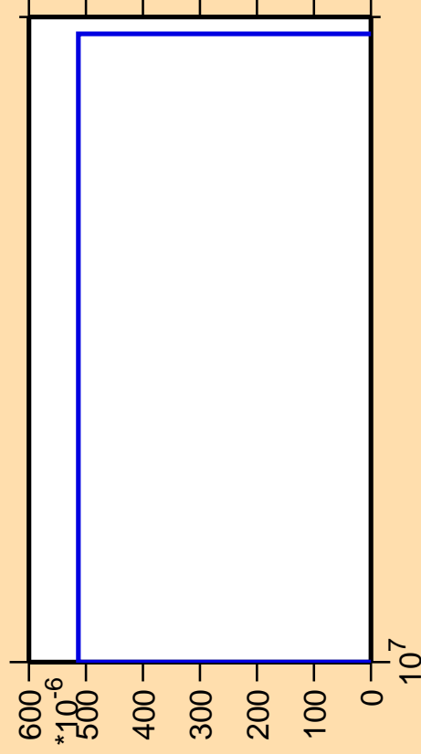
\Delta\sigma/\sigma vs. E for ^{226}\text{Pa} (mt 11)
