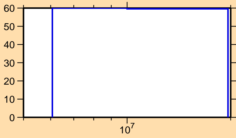
\Delta\sigma/\sigma vs. E for ^{226}\text{Pa}(n,2n)
