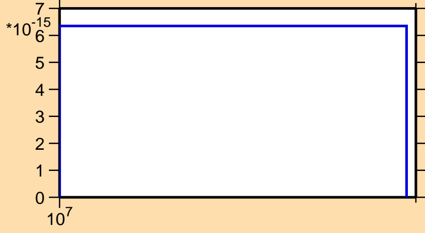
\sigma vs. E for ^{226}\text{Pa} (mt 34)
