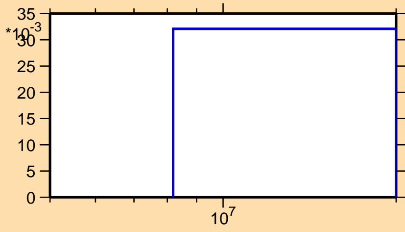
\sigma vs. E for ^{226}\text{Pa}(n,3n)
