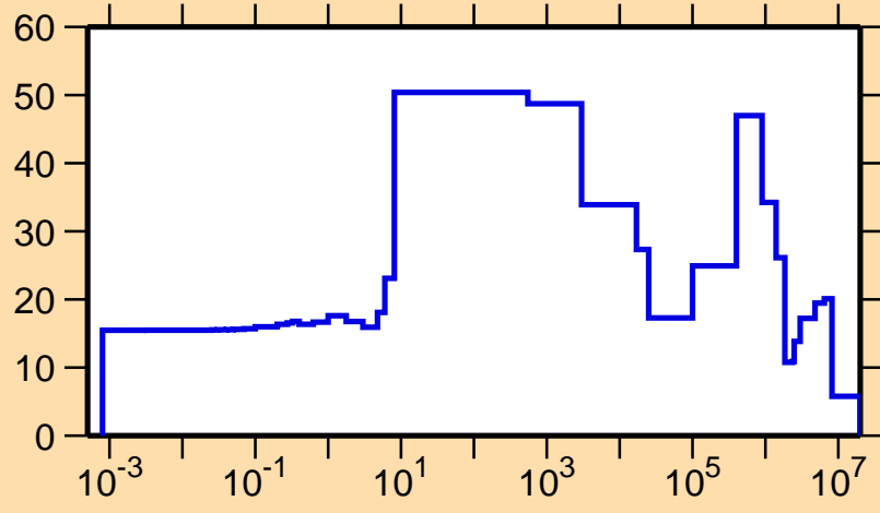
\Delta\sigma/\sigma vs. E for ^{226}\text{Pa}(n,\text{el.})
