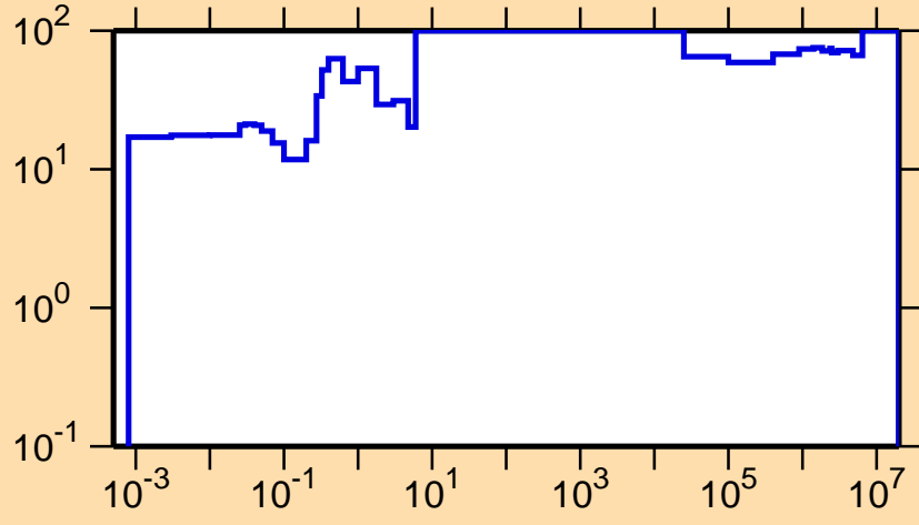
\Delta\sigma/\sigma vs. E for ^{226}\text{Pa}(n,\gamma)
