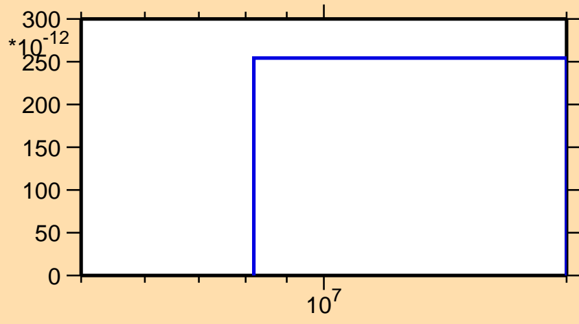
\sigma vs. E for ^{226}\text{Pa}(n,\text{He}3)
