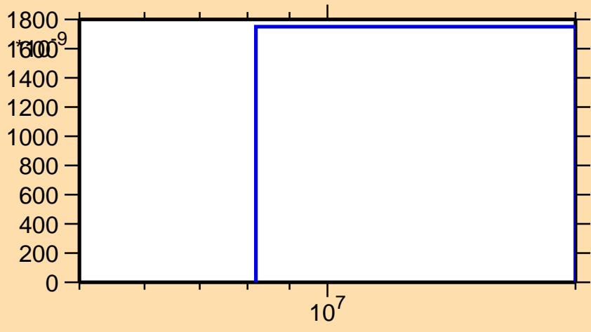
\sigma vs. E for ^{226}\text{Pa}(n,\text{nd})
