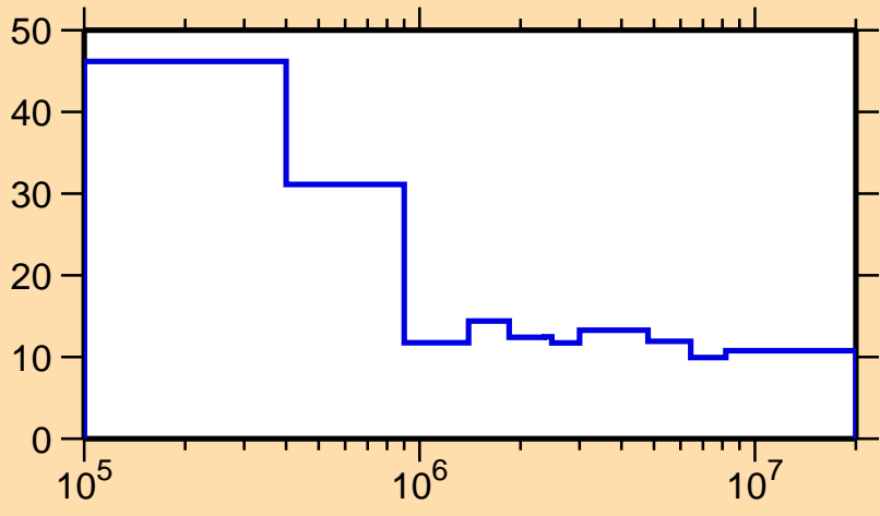
\Delta\sigma/\sigma vs. E for ^{226}\text{Pa}(n,\text{nonel.})
