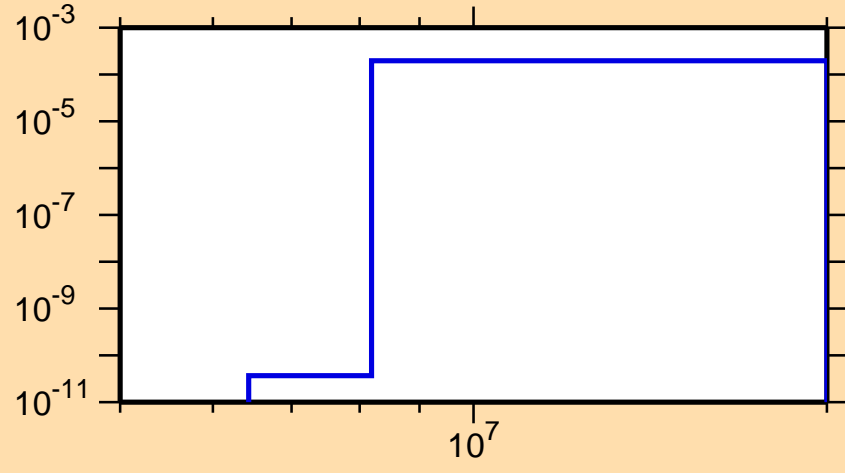
\sigma vs. E for ^{226}\text{Pa}(n,t)
