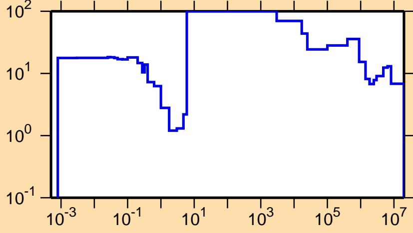
\Delta\sigma/\sigma vs. E for ^{226}\text{Pa}(n,\text{tot.})
