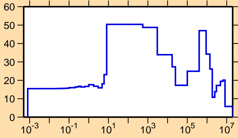
\Delta\sigma/\sigma vs. E for ^{226}\text{Pa}(n,\text{el.})
