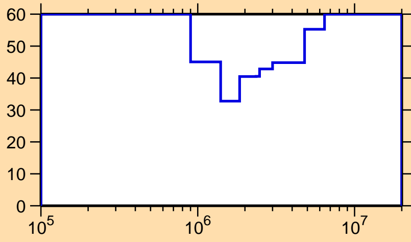
\Delta\sigma/\sigma vs. E for ^{226}\text{Pa}(n,\text{inel.})
