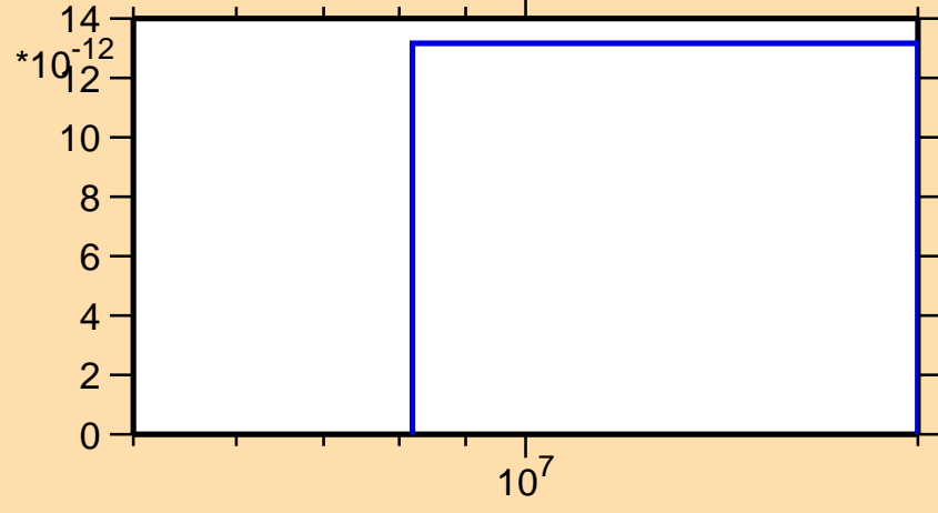
\sigma vs. E for ^{226}\text{Pa}(\text{mt117})
