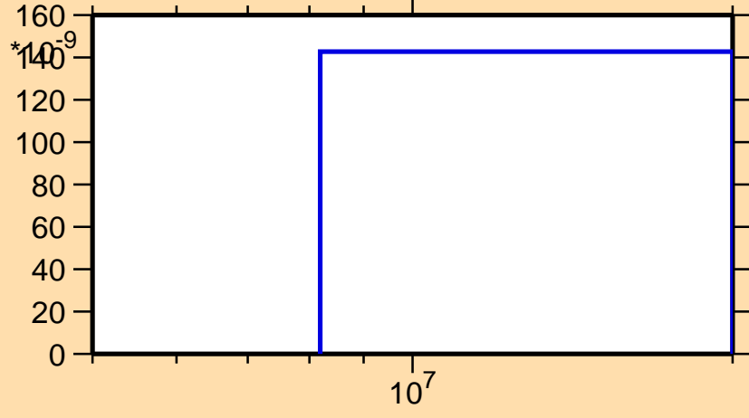
\sigma vs. E for ^{226}\text{Pa}(n,nt)
