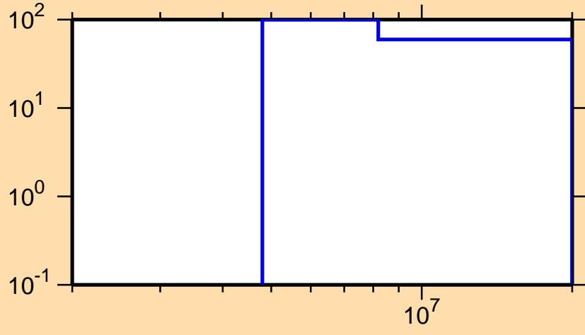
\Delta\sigma/\sigma vs. E for ^{226}\text{Pa}(n,2n)
