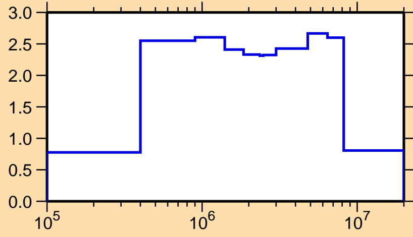
\sigma vs. E for ^{226}\text{Pa}(n,n\text{cont.})
