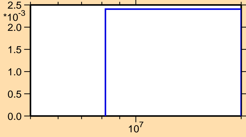
\sigma vs. E for ^{226}\text{Pa}(n,3n\alpha)
