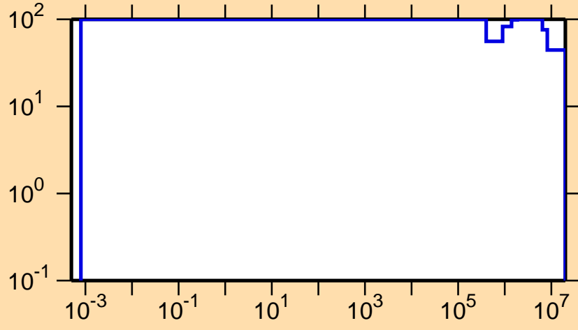
\Delta\sigma/\sigma vs. E for ^{226}\text{Pa}(n,p)
