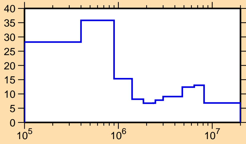
\Delta\sigma/\sigma vs. E for ^{226}\text{Pa}(n,\text{tot.})
