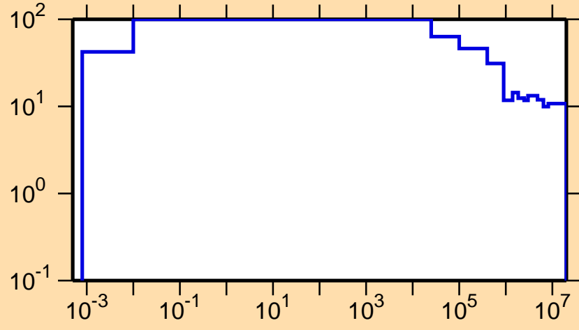
\Delta\sigma/\sigma vs. E for ^{226}\text{Pa}(n,\text{nonel.})
