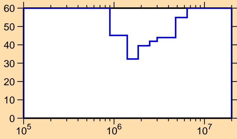
\Delta\sigma/\sigma vs. E for ^{226}\text{Pa}(n,n\text{cont.})
