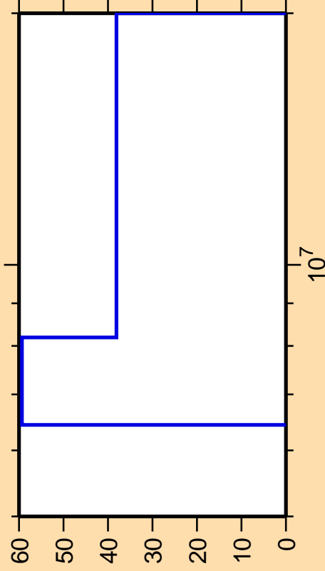
\Delta\sigma/\sigma vs. E for ^{226}\text{Pa}(n,t)
