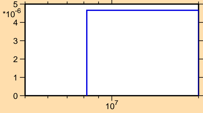
\sigma vs. E for ^{226}\text{Pa}(n,2np)
