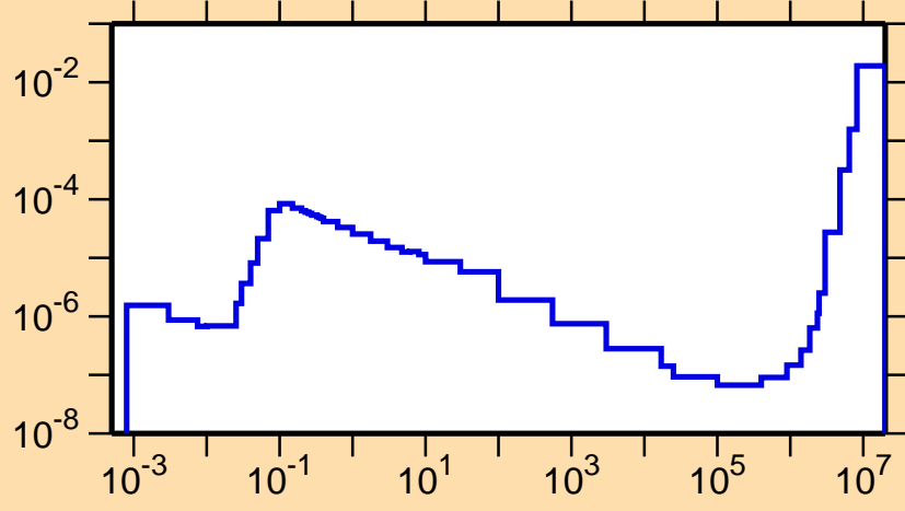
\sigma vs. E for ^{226}\text{Pa}(n,p)
