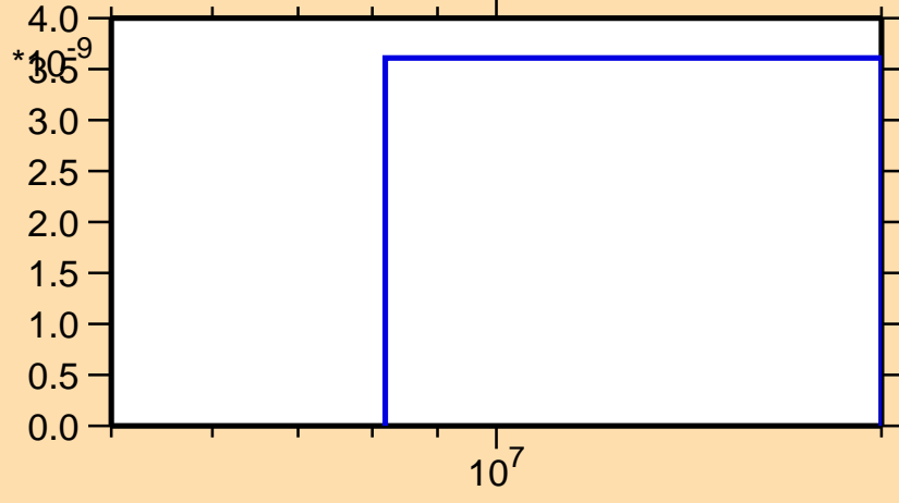
\sigma vs. E for ^{226}\text{Pa}(n,p\alpha)
