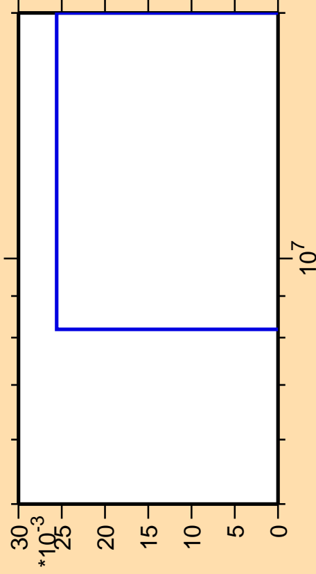
\Delta\sigma/\sigma vs. E for ^{226}\text{Pa}(\text{mt } 34)
