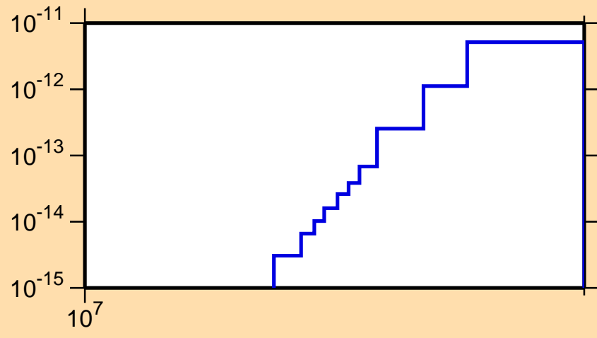
\sigma vs. E for ^{227}\text{Pa}(\text{mt117})
