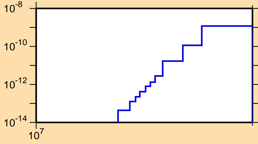
\sigma vs. E for ^{227}\text{Pa}(n,\text{He}3)
