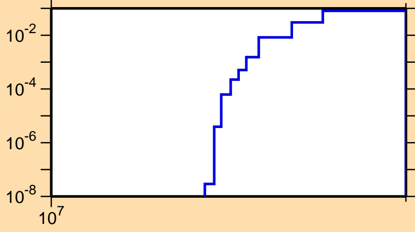
\sigma vs. E for ^{227}\text{Pa}(n,3n)
