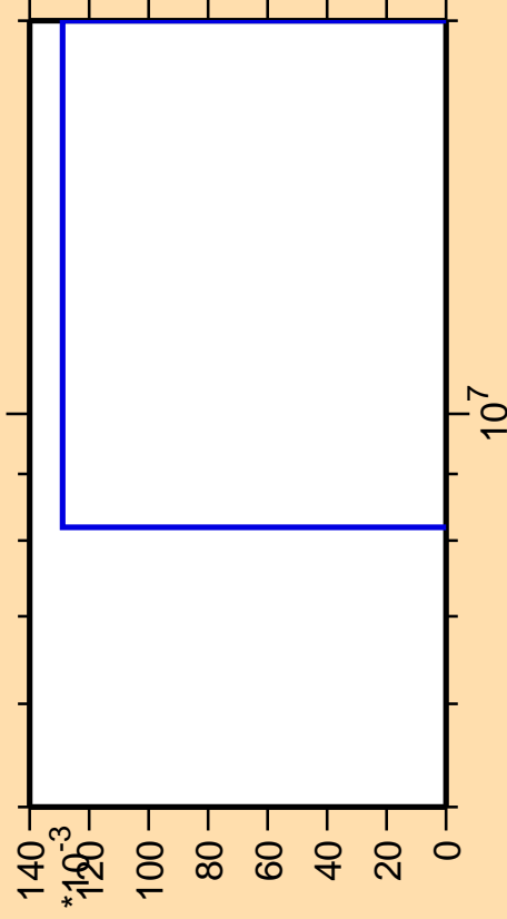
\Delta\sigma/\sigma vs. E for ^{227}\text{Pa} (mt 45)
