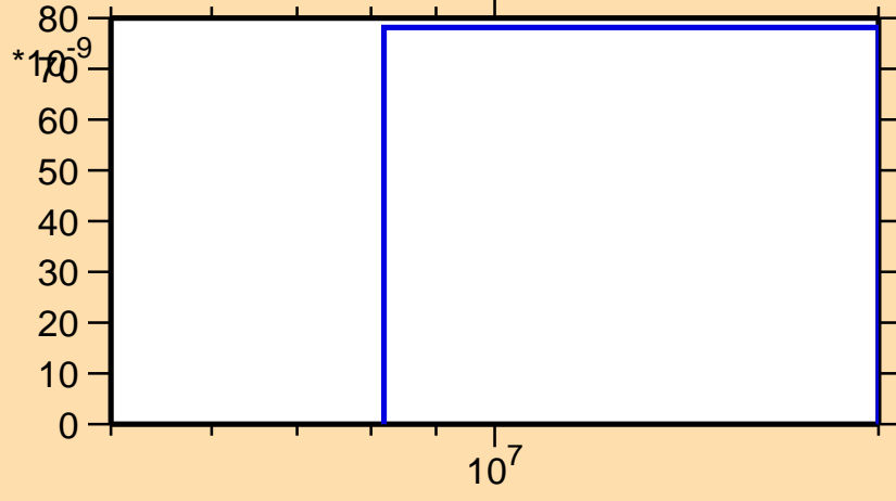
\sigma vs. E for ^{227}\text{Pa}(n,2n\alpha)
