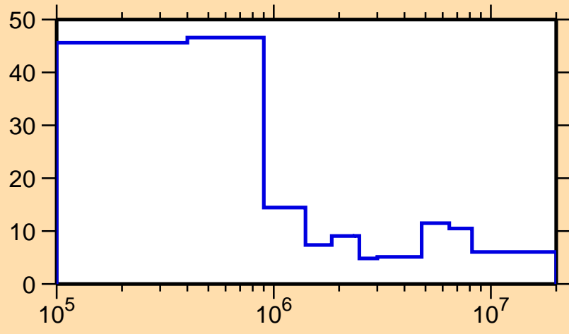
\Delta\sigma/\sigma vs. E for ^{227}\text{Pa}(n,\text{tot.})
