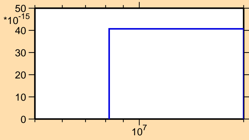
\sigma vs. E for ^{227}\text{Pa} (mt 45)
