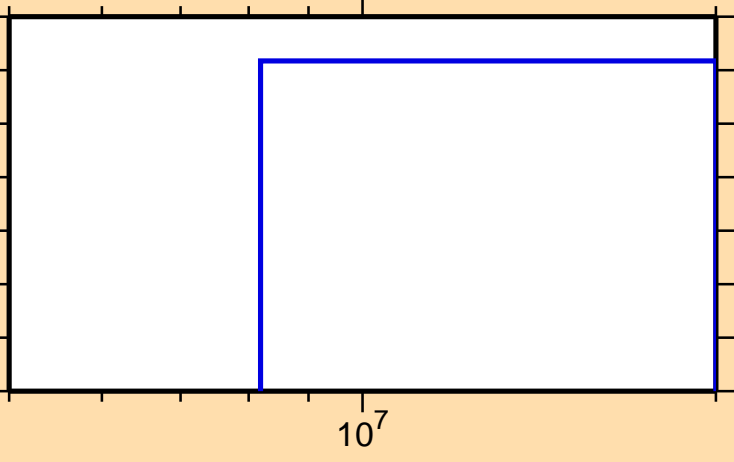
\sigma vs. E for ^{227}\text{Pa}(n,nt)
