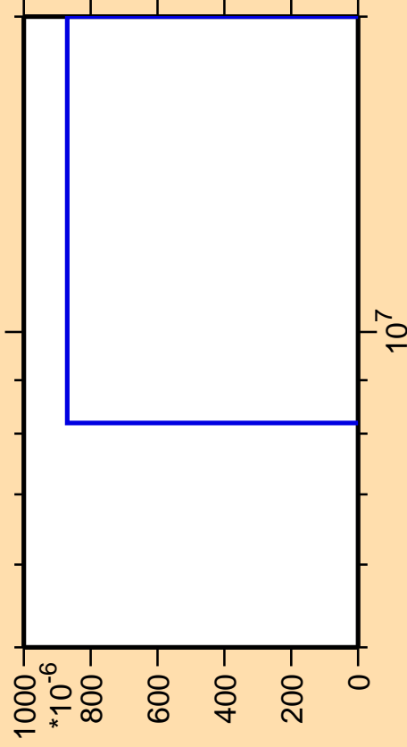
\Delta\sigma/\sigma vs. E for ^{227}\text{Pa}(\text{mt } 34)
