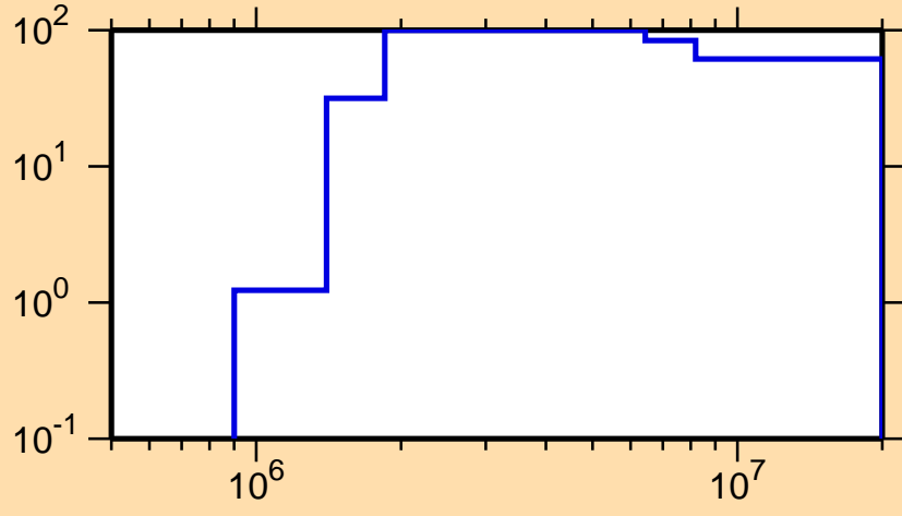
\Delta\sigma/\sigma vs. E for ^{227}\text{Pa}(n,p)
