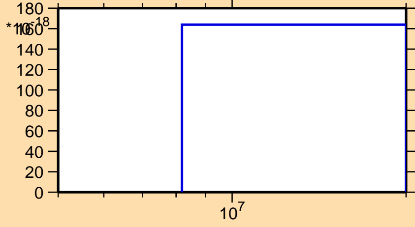
\sigma vs. E for ^{227}\text{Pa}(\text{mt } 34)
