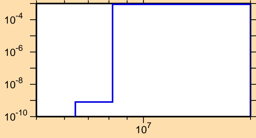
\sigma vs. E for ^{227}\text{Pa}(n,np)
