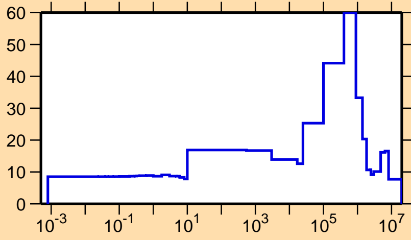
\Delta\sigma/\sigma vs. E for ^{227}\text{Pa}(n,el.)
