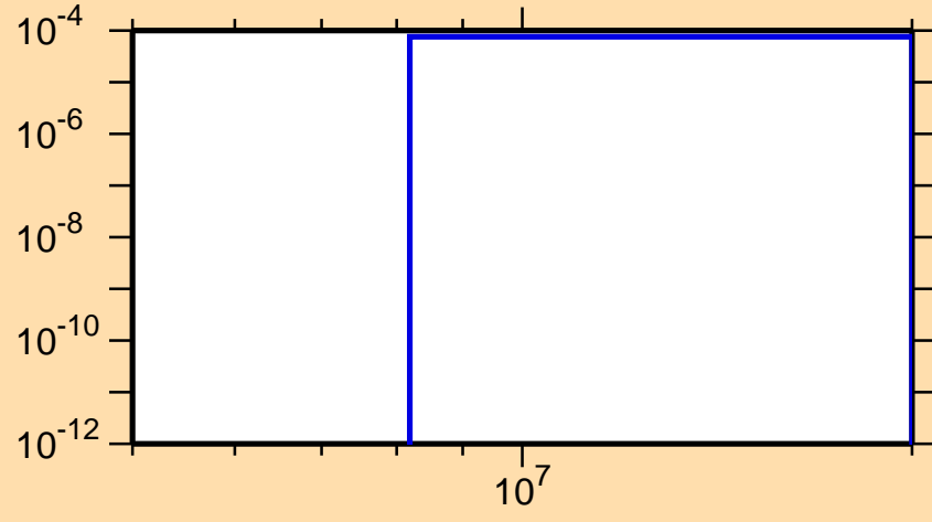
\sigma vs. E for ^{227}\text{Pa}(n,t)
