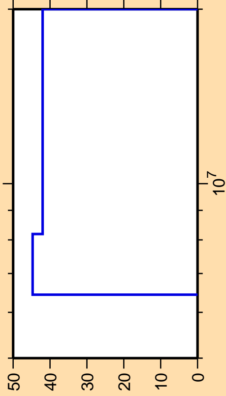
\Delta\sigma/\sigma vs. E for ^{227}\text{Pa}(n,n_1)
