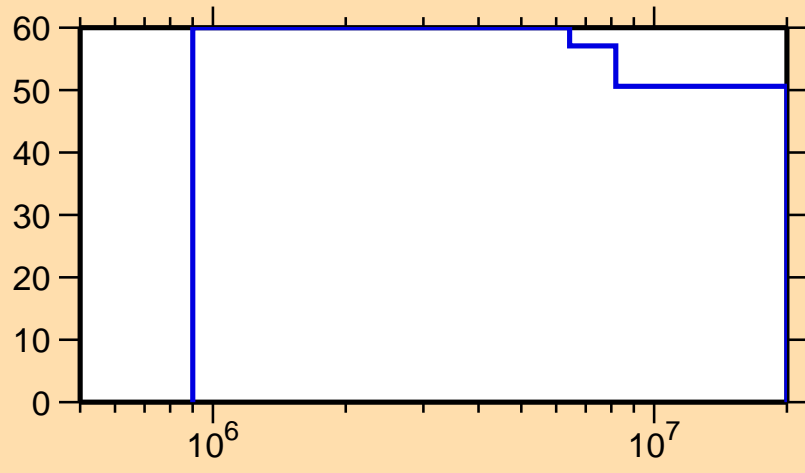
\Delta\sigma/\sigma vs. E for ^{227}\text{Pa}(n,n\text{cont.})
