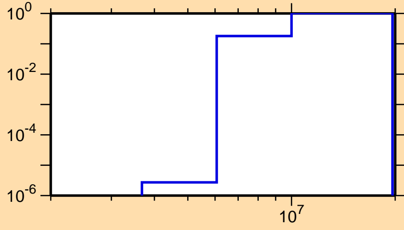
\sigma vs. E for ^{228}\text{Pa}(n,2n)
