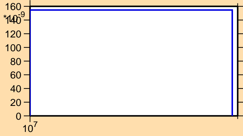
\sigma vs. E for ^{228}\text{Pa}(n,\text{nd})
