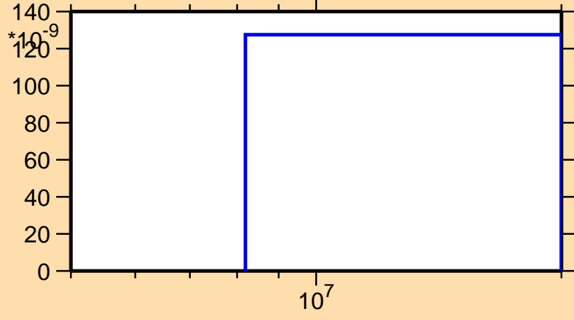
\sigma vs. E for ^{228}\text{Pa}(n,\text{nd})
