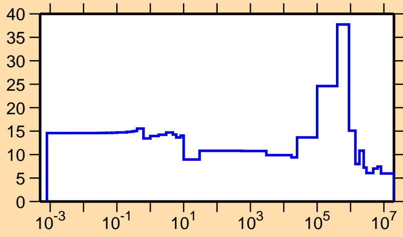
\Delta\sigma/\sigma vs. E for ^{228}\text{Pa}(n,el.)
