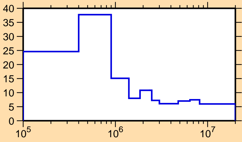
\Delta\sigma/\sigma vs. E for ^{228}\text{Pa}(n,\text{el.})
