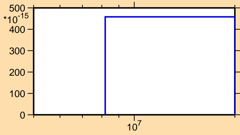
\sigma vs. E for ^{228}\text{Pa}(n,3n\alpha)
