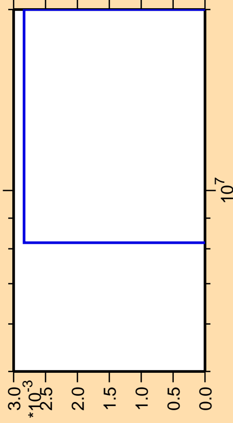
\Delta\sigma/\sigma vs. E for ^{228}\text{Pa} (mt 34)
