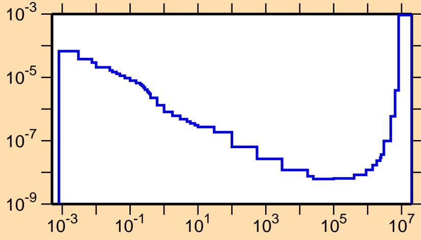
\sigma vs. E for ^{228}\text{Pa}(n,\alpha)
