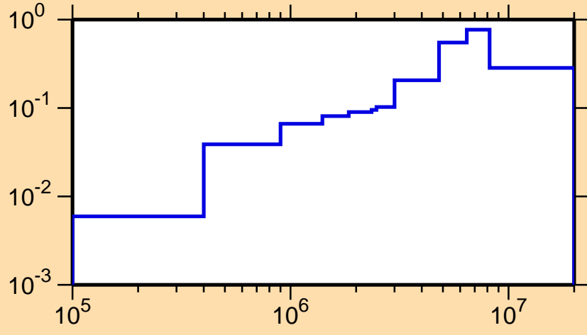
\sigma vs. E for ^{228}\text{Pa}(n,n\text{cont.})
