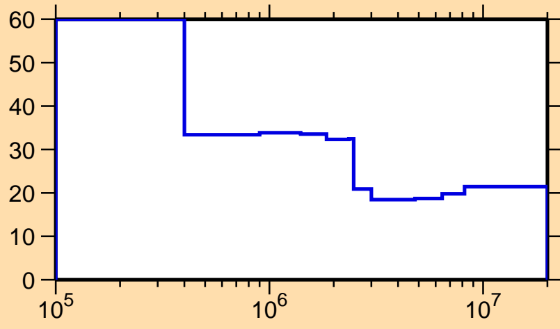
\Delta\sigma/\sigma vs. E for ^{228}\text{Pa}(n,f)
