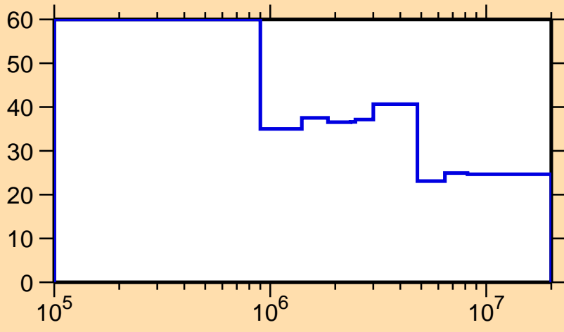
\Delta\sigma/\sigma vs. E for ^{228}\text{Pa}(n,n_1)
