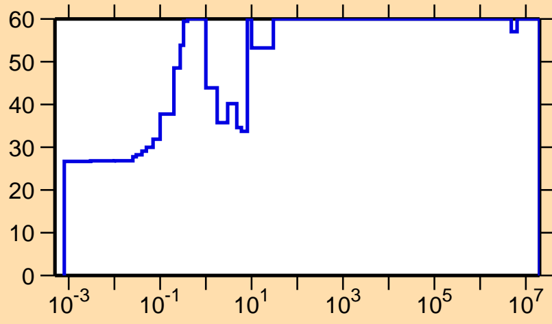
\Delta\sigma/\sigma vs. E for ^{228}\text{Pa}(n,\gamma)
