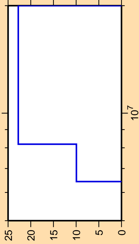
\Delta\sigma/\sigma vs. E for ^{228}\text{Pa}(n,t)
