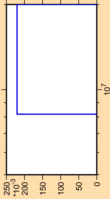
\Delta\sigma/\sigma vs. E for ^{228}\text{Pa}(\text{mt117})
