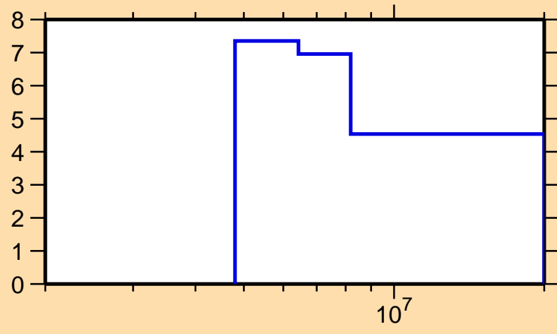
\Delta\sigma/\sigma vs. E for ^{228}\text{Pa}(n,\text{tot.})
