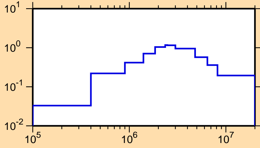
\sigma vs. E for ^{228}\text{Pa}(n,n_1)
