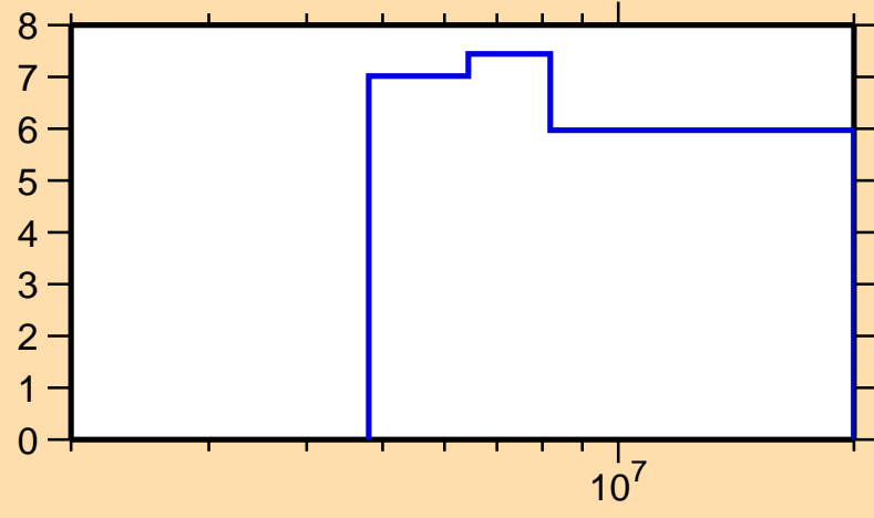
\Delta\sigma/\sigma vs. E for ^{228}\text{Pa}(n,\text{el.})
