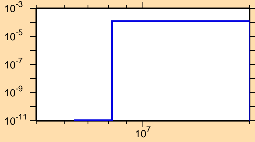
\sigma vs. E for ^{228}\text{Pa}(n,t)
