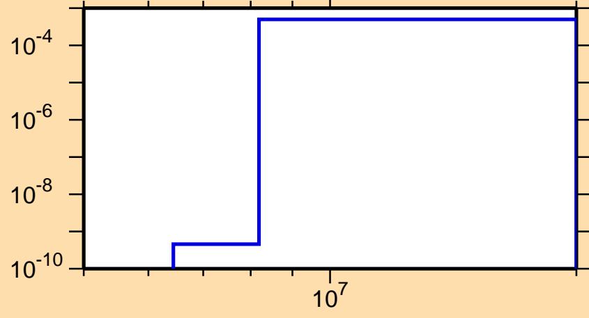
\sigma vs. E for ^{228}\text{Pa}(n,np)
