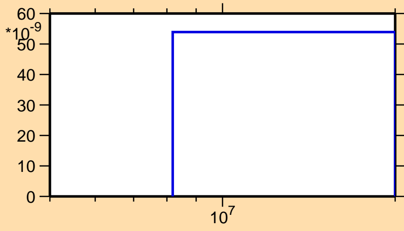
\sigma vs. E for ^{228}\text{Pa}(n,nt)
