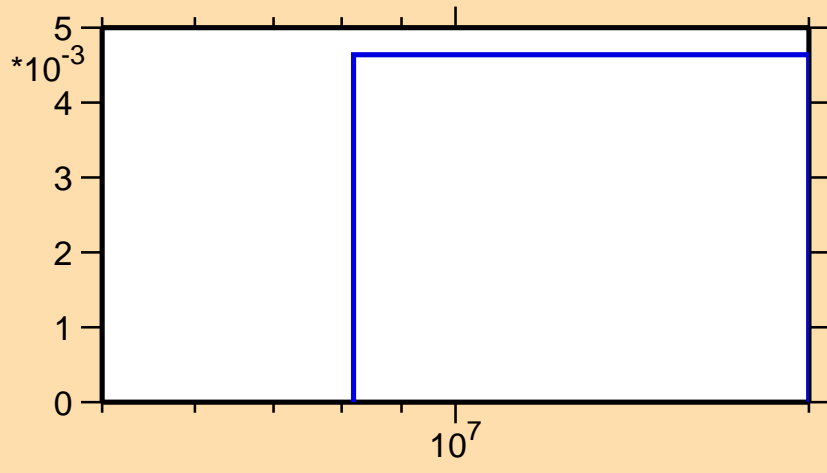
\sigma vs. E for ^{228}\text{Pa}(n,3n)
