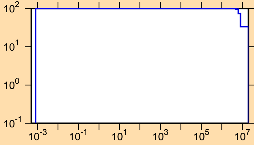
\Delta\sigma/\sigma vs. E for ^{228}\text{Pa}(n,p)
