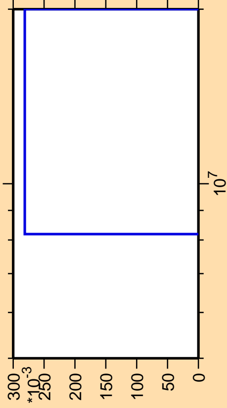
\Delta\sigma/\sigma vs. E for ^{228}\text{Pa} (mt 45)
