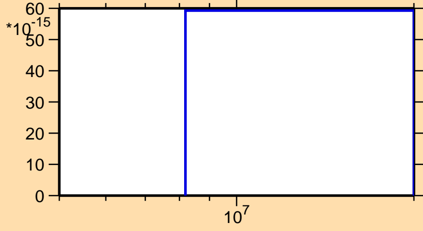
\sigma vs. E for ^{228}\text{Pa} (mt 45)
