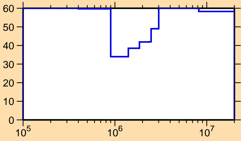
\Delta\sigma/\sigma vs. E for ^{228}\text{Pa}(n,\text{inel.})
