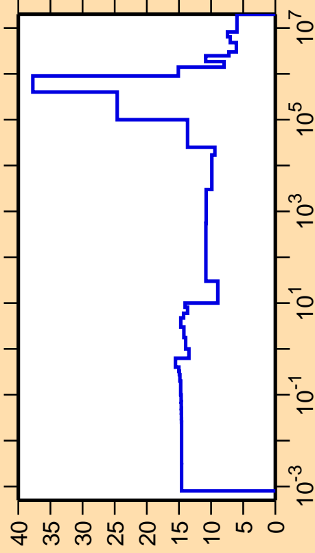
\Delta\sigma/\sigma vs. E for ^{228}\text{Pa}(n,\text{el.})
