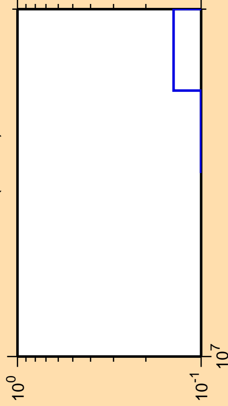
\Delta\sigma/\sigma vs. E for ^{229}\text{Pa} (mt 11)
