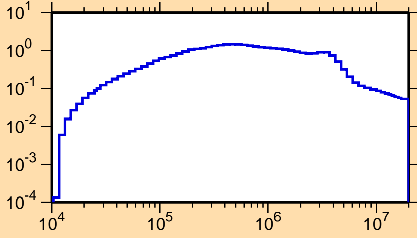
\sigma vs. E for ^{229}\text{Pa}(n,\text{inel.})
