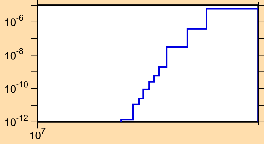
\sigma vs. E for ^{229}\text{Pa}(n,nd)
