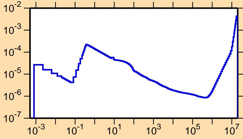
\sigma vs. E for ^{229}\text{Pa}(n,\alpha)
