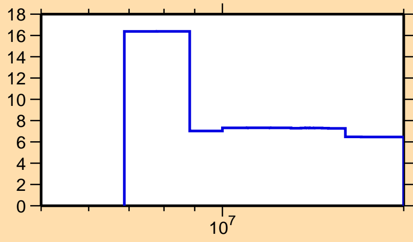
\Delta\sigma/\sigma vs. E for ^{229}\text{Pa}(n,\text{el.})
