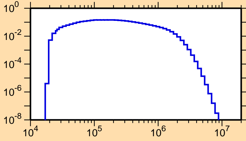
\sigma vs. E for ^{229}\text{Pa}(n,n_2)
