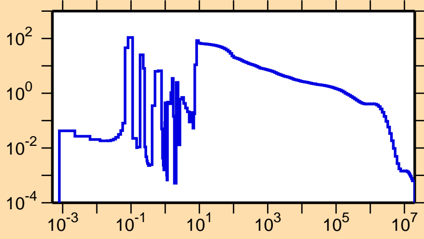
\sigma vs. E for ^{229}\text{Pa}(n,\gamma)
