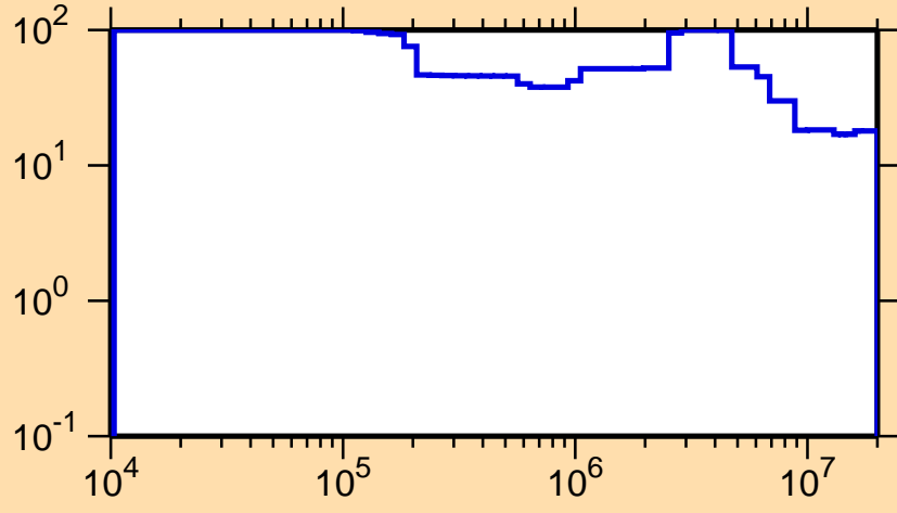
\Delta\sigma/\sigma vs. E for ^{229}\text{Pa}(n,f)
