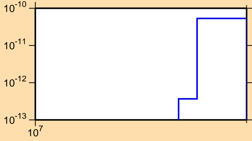
\sigma vs. E for ^{229}\text{Pa}(n,3n\alpha)
