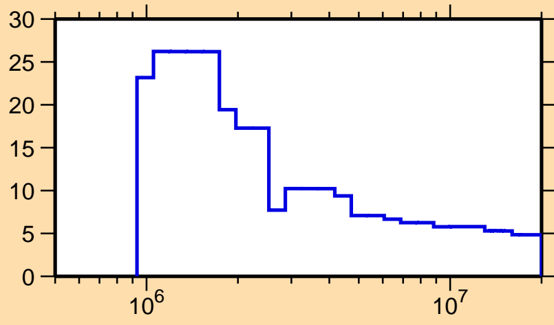
\Delta\sigma/\sigma vs. E for ^{229}\text{Pa}(n,\text{nonel.})
