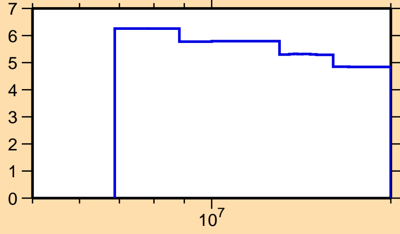
\Delta\sigma/\sigma vs. E for ^{229}\text{Pa}(n,\text{nonel.})
