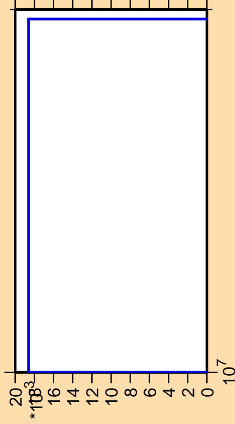
\Delta\sigma/\sigma vs. E for ^{229}\text{Pa} (mt 45)
