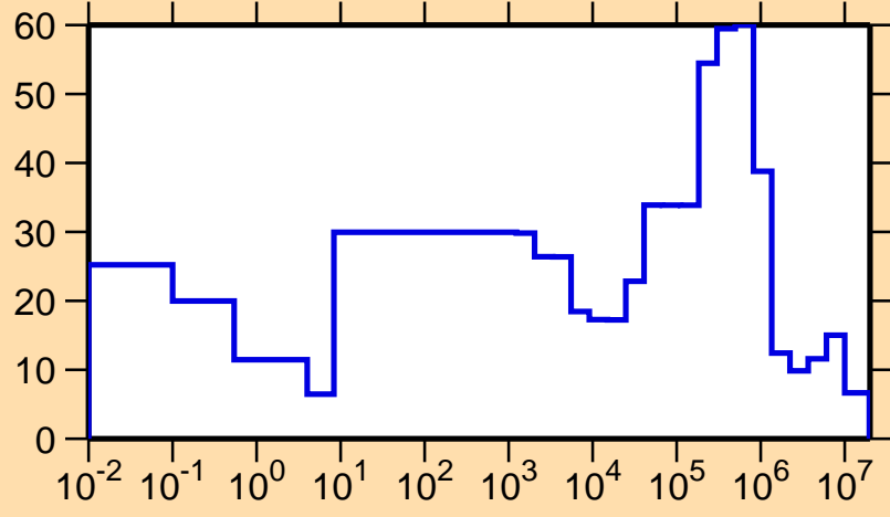
\Delta\sigma/\sigma vs. E for ^{229}\text{Pa}(n,el.)
