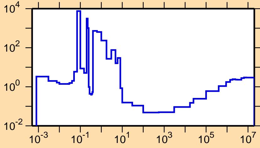
\sigma vs. E for ^{229}\text{Pa}(n,f)
