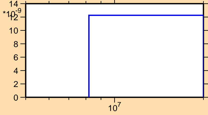
\sigma vs. E for ^{229}\text{Pa}(n,2np)
