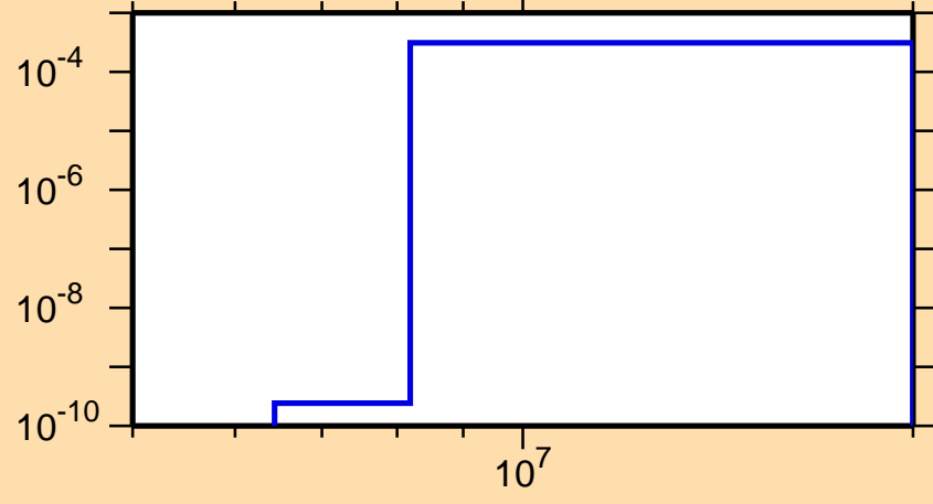
\sigma vs. E for ^{229}\text{Pa}(n,d)
